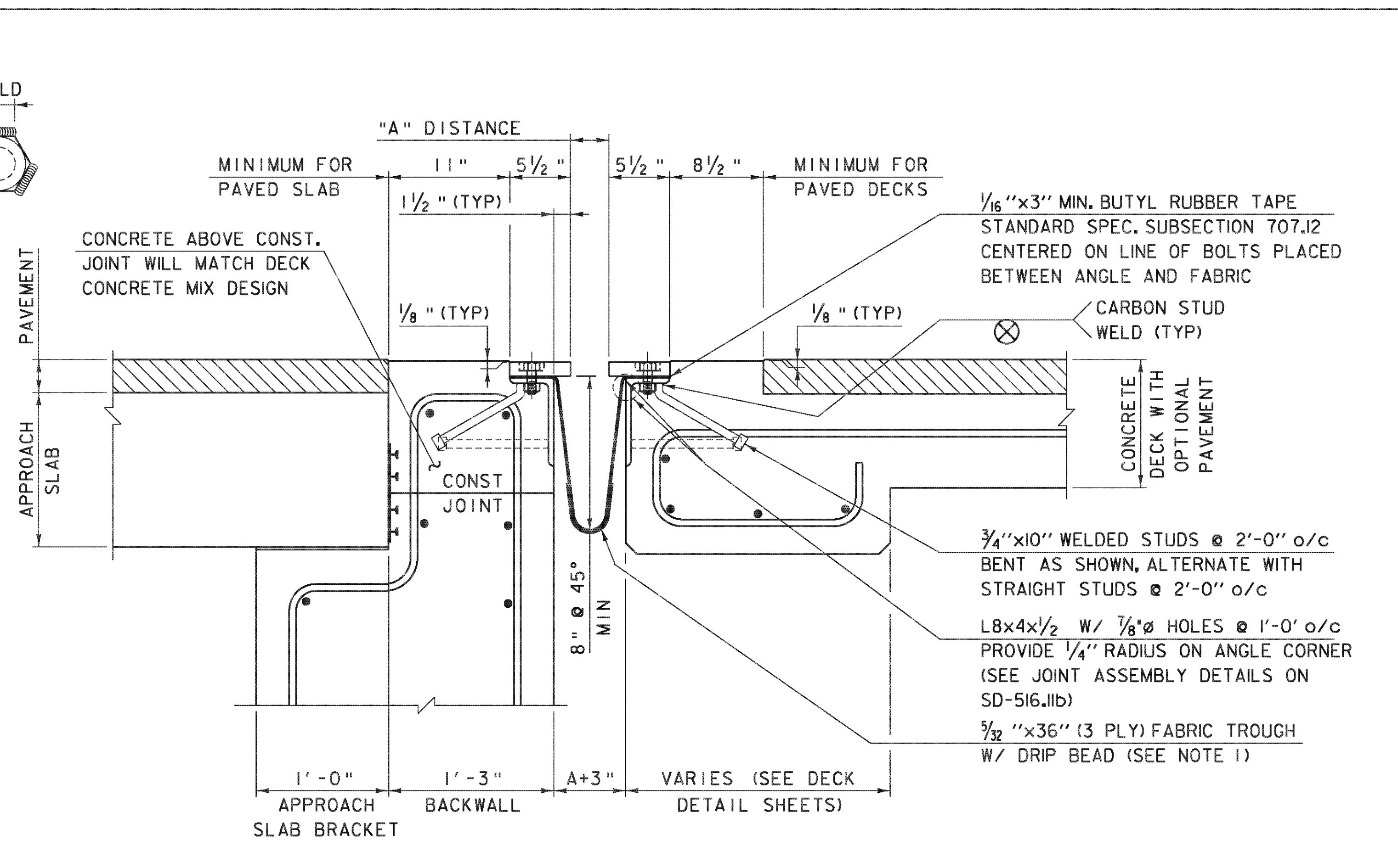
TYPICAL SECTION BETWEEN GIRDERS SCALE 1/2" = 1'-0"
