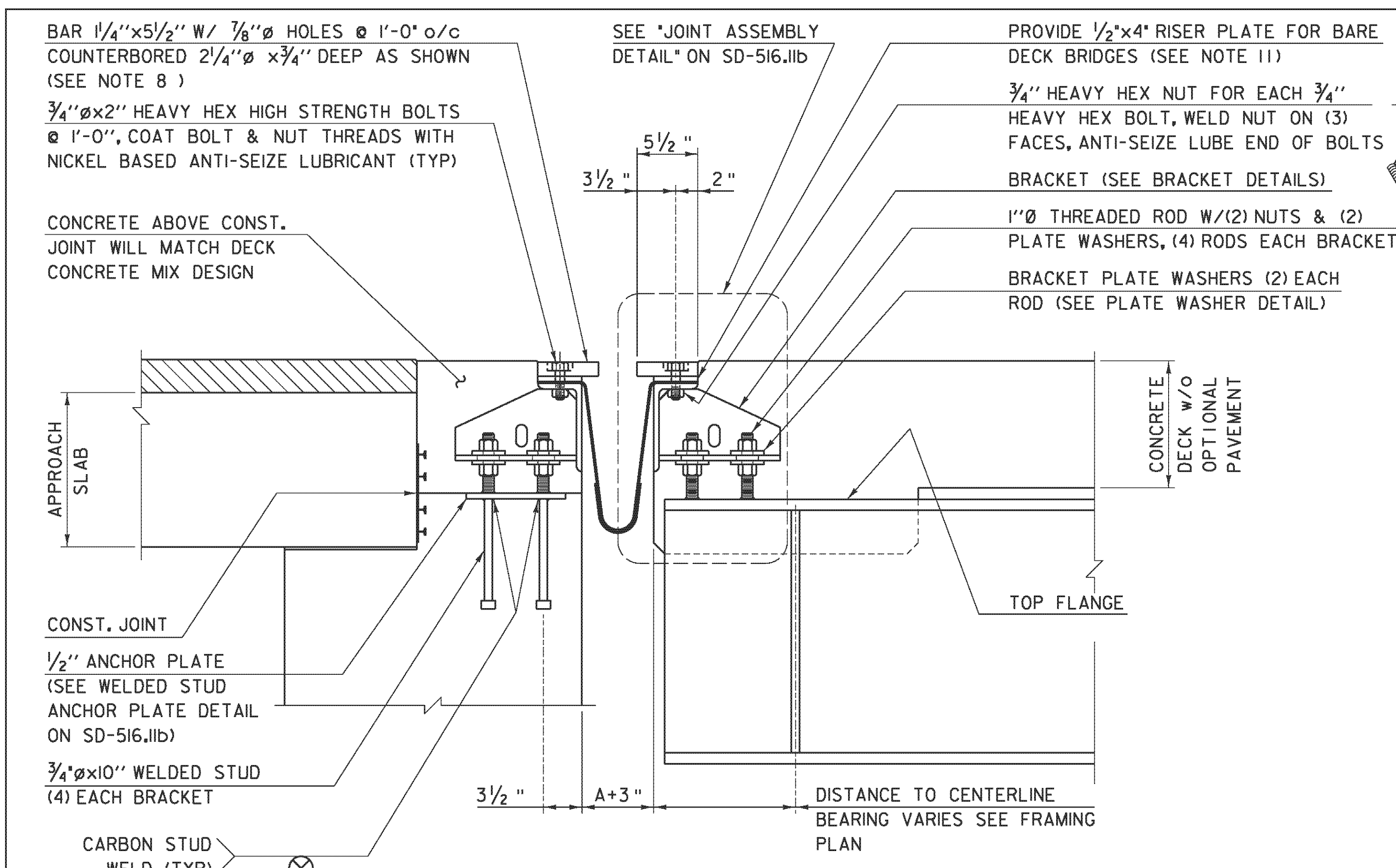
TYPICAL SECTION AT GIRDERS SCALE 1/2" = 1'-0"
