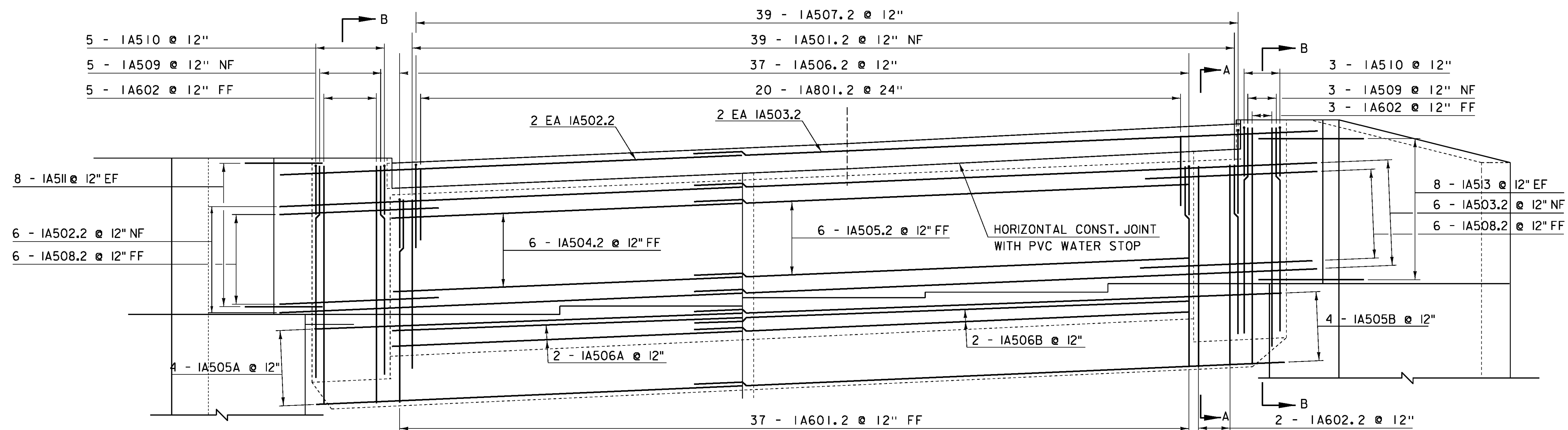
ABUTMENT #1 BACK WALL ELEVATION
