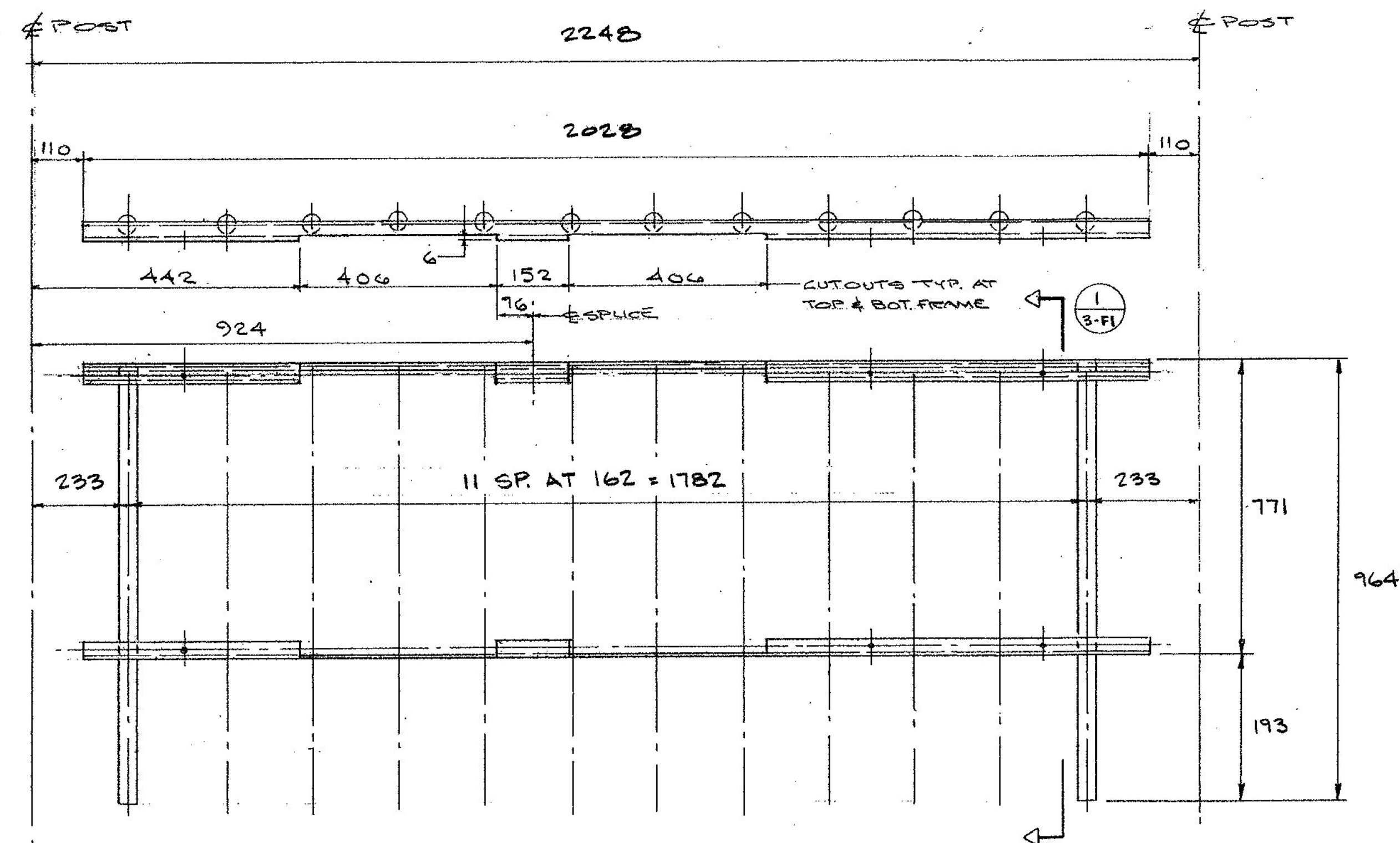
SPINDLE PANEL "PP2" (2 REQ'D.)
