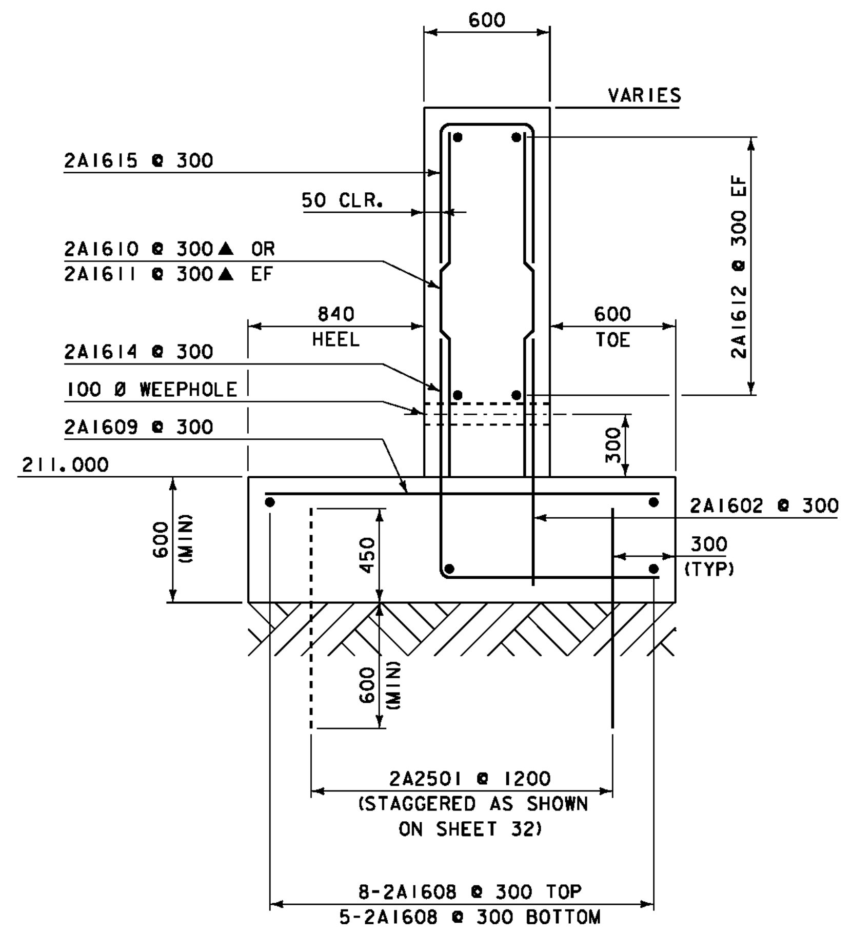
ABUTMENT #2 SHORT TYPICAL SECTION SCALE 1:20
