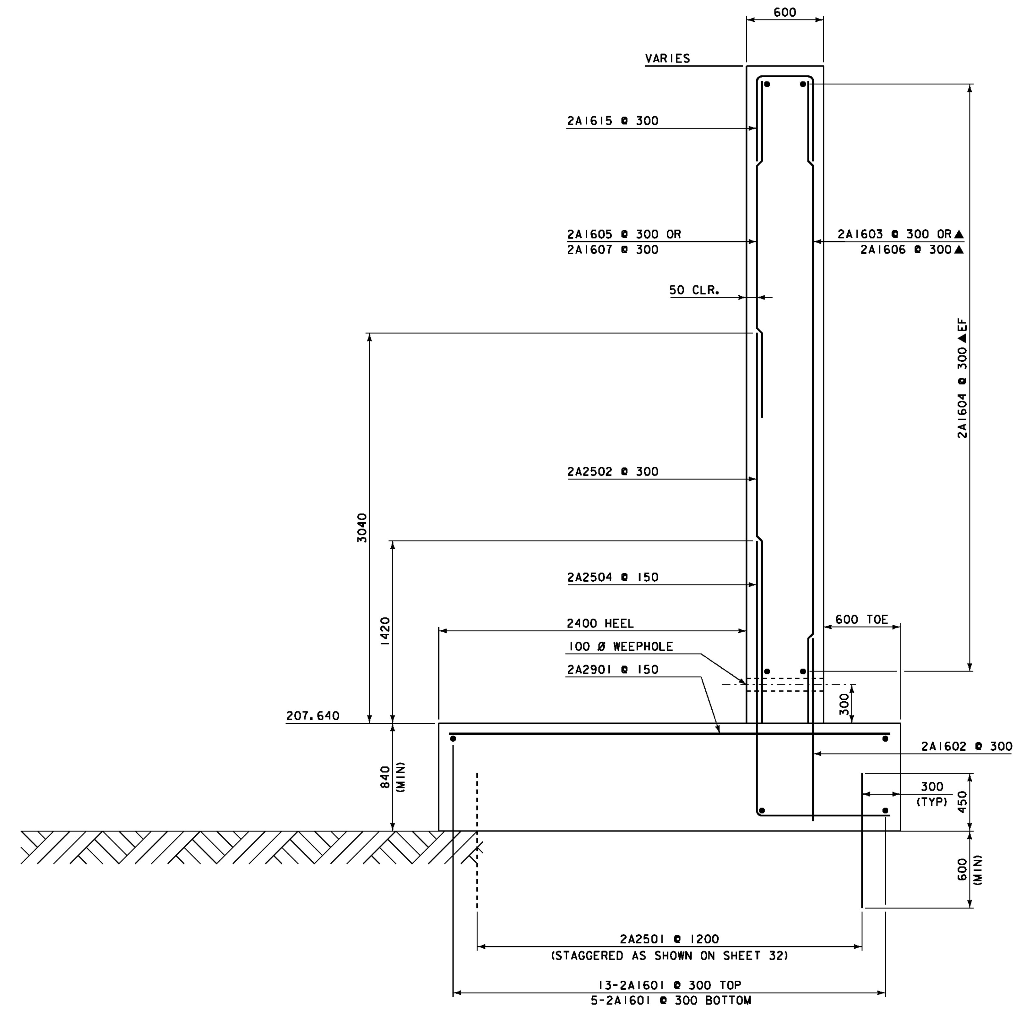
ABUTMENT #2 TALL TYPICAL SECTION SCALE 1:20
