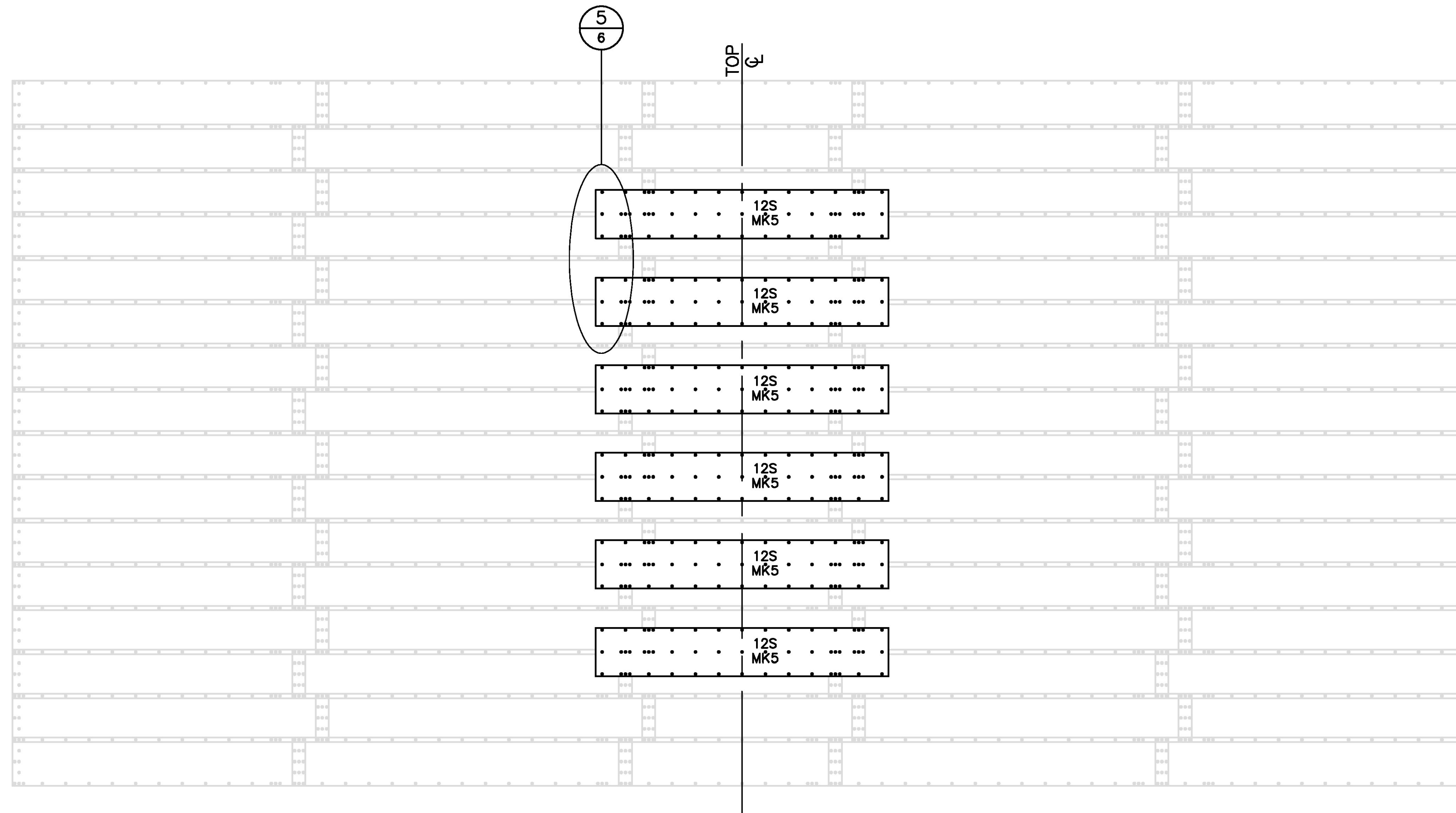
RIB PLATE LAYOUT - OUTSIDE FLAT VIEW
