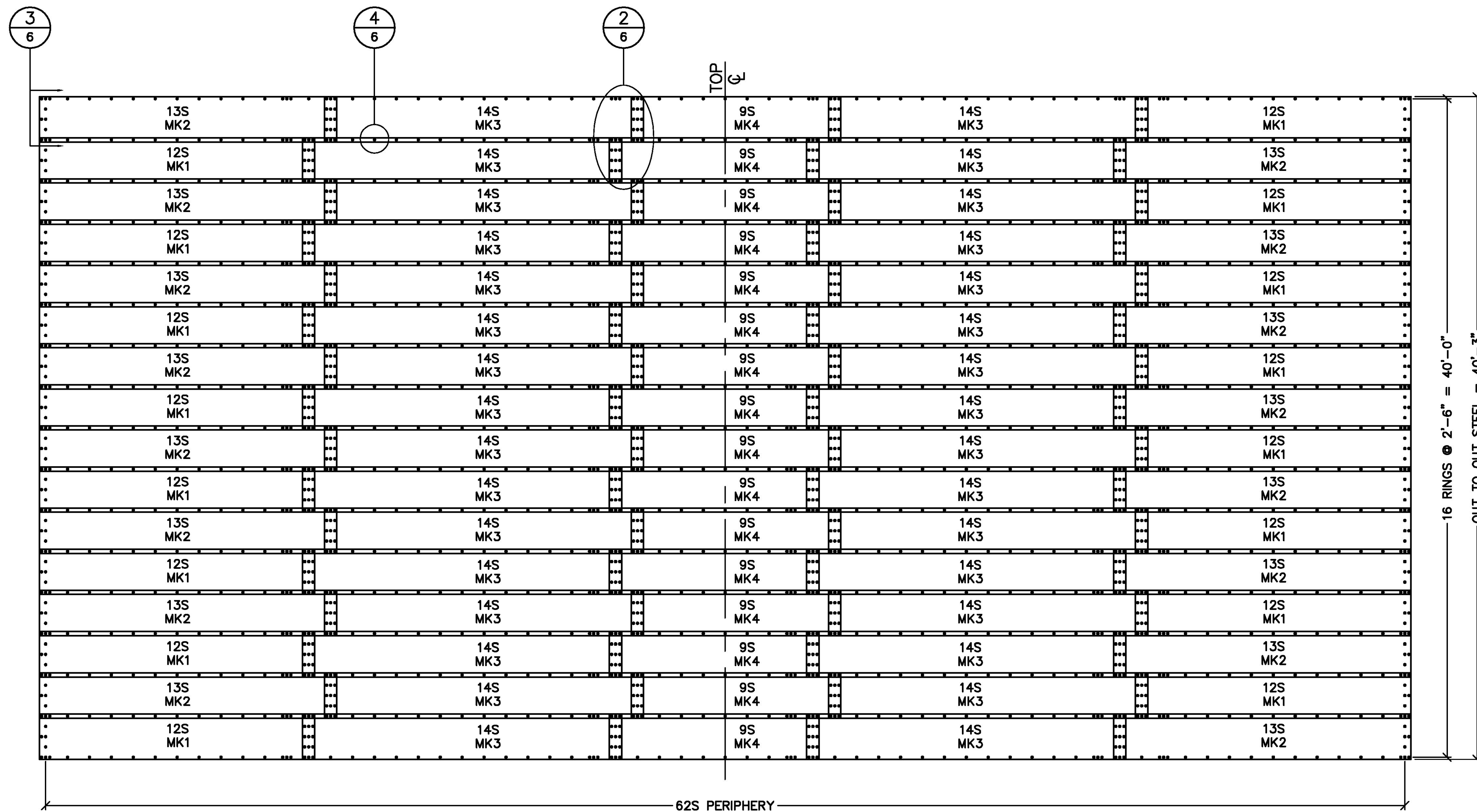
STRUCTURE LAYOUT - OUTSIDE FLAT VIEW
