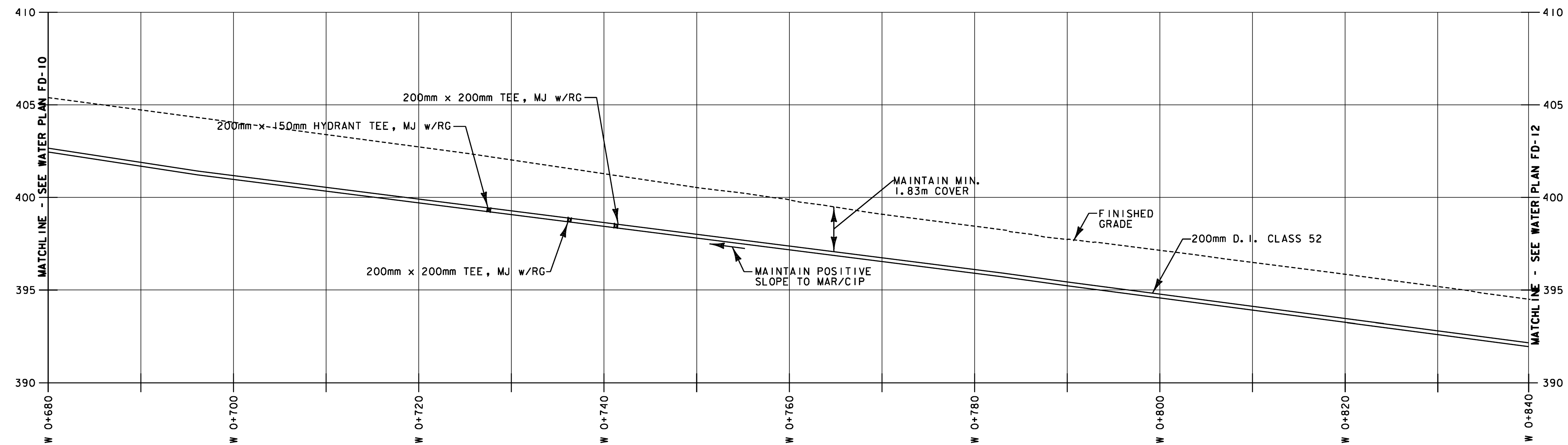
WATER MAIN PROFILE 0 10 20 HORIZONTAL SCALE 1:250 0 5 10 VERTICAL SCALE 1:125
