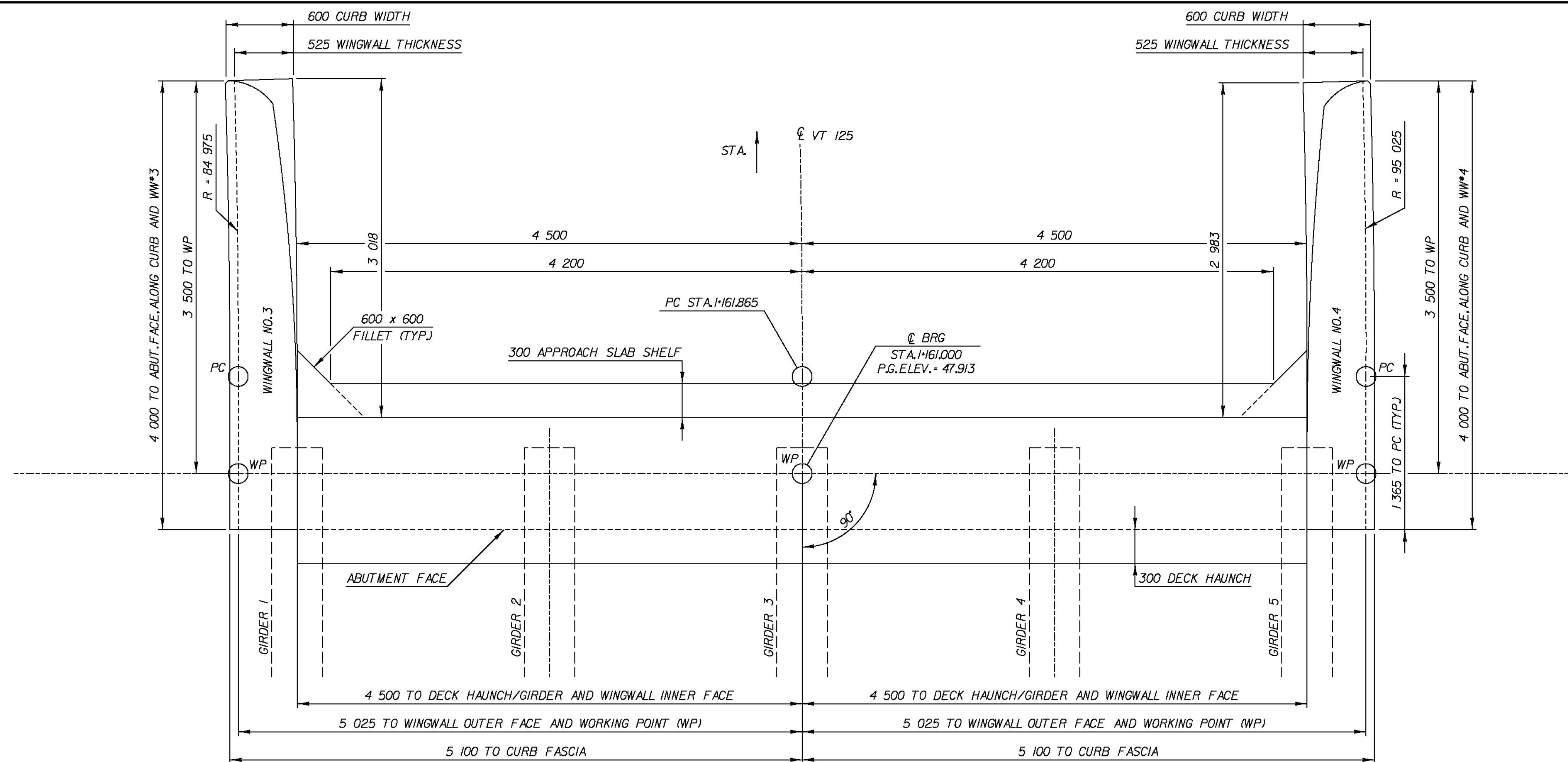
ABUTMENT NO.2 PLAN
