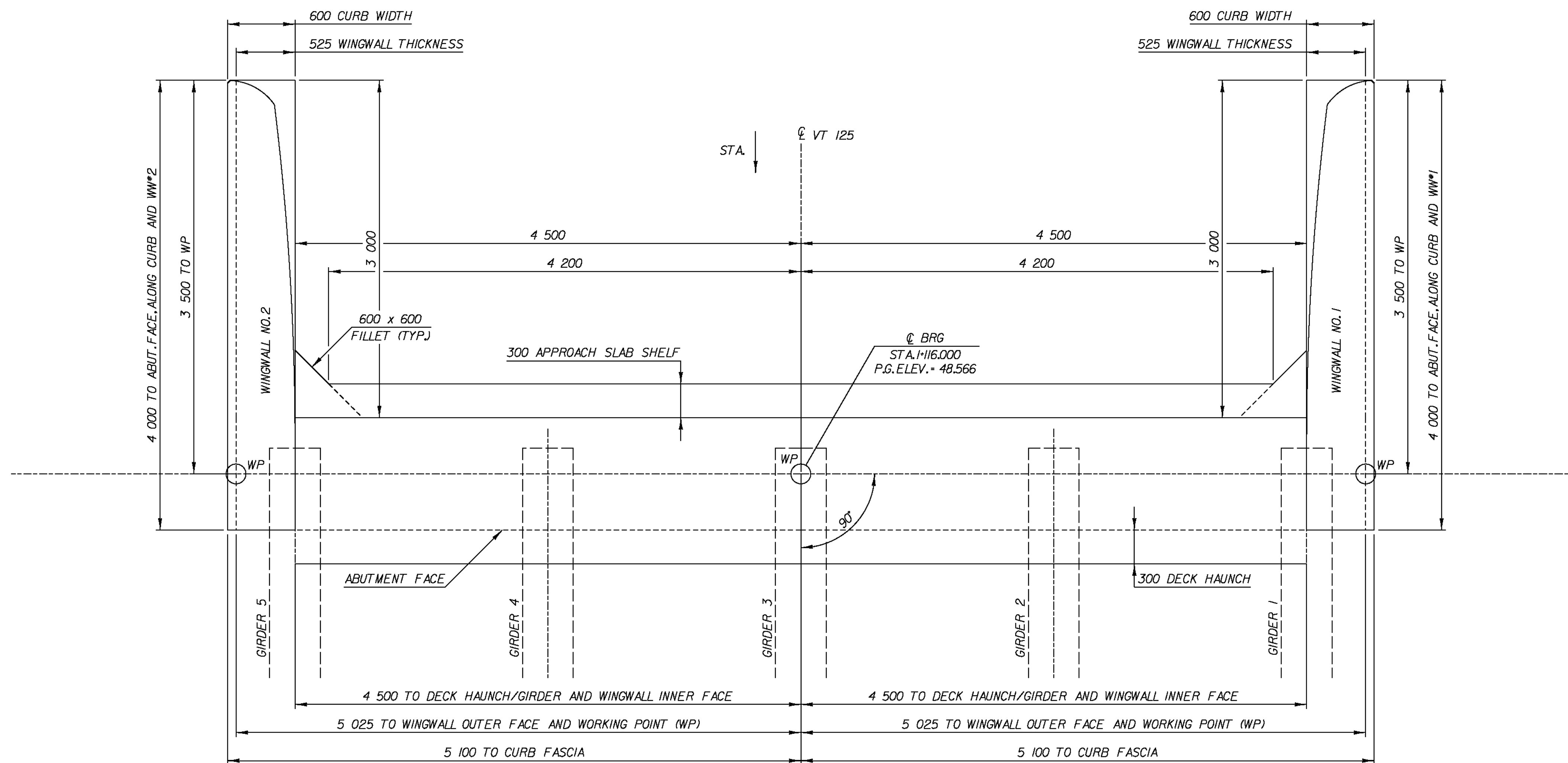
ABUTMENT NO. 1 PLAN
