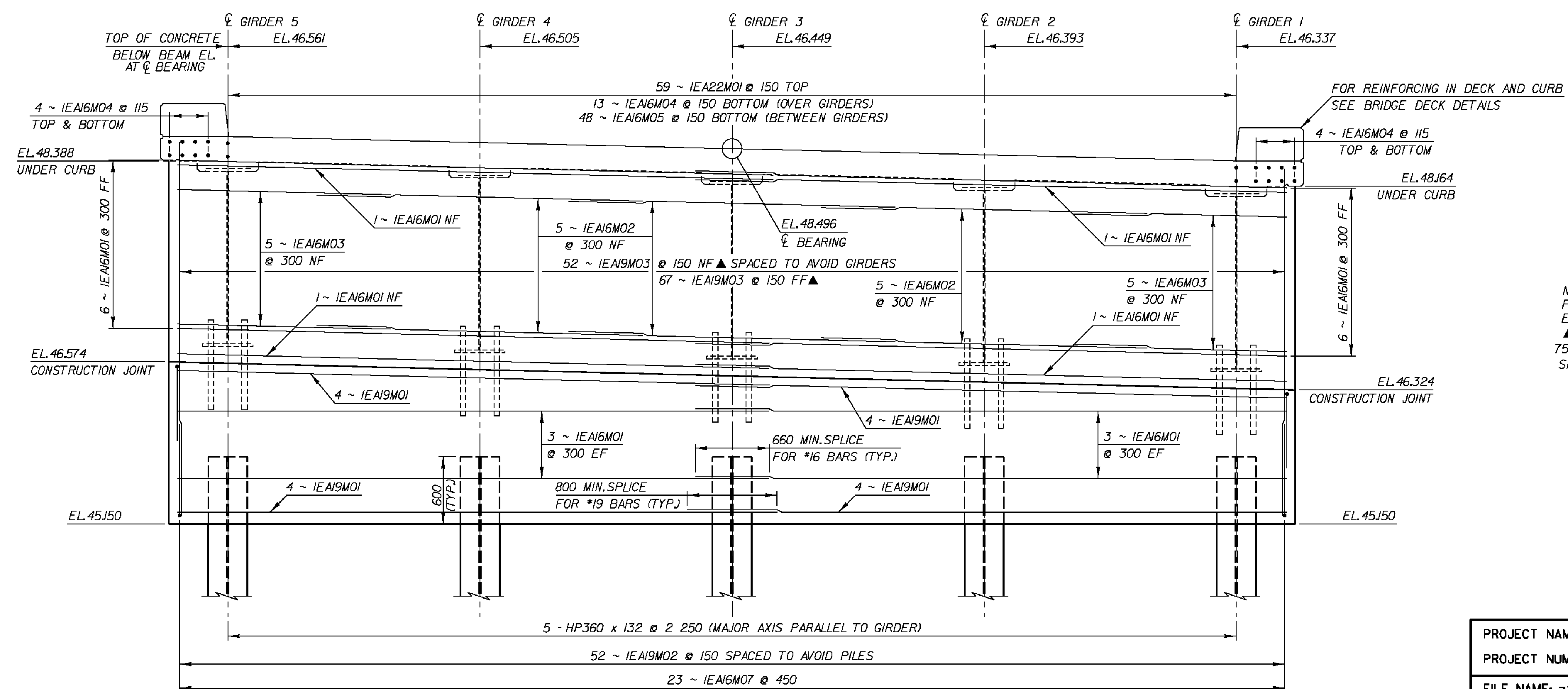
ABUTMENT NO. 1 ELEVATION
