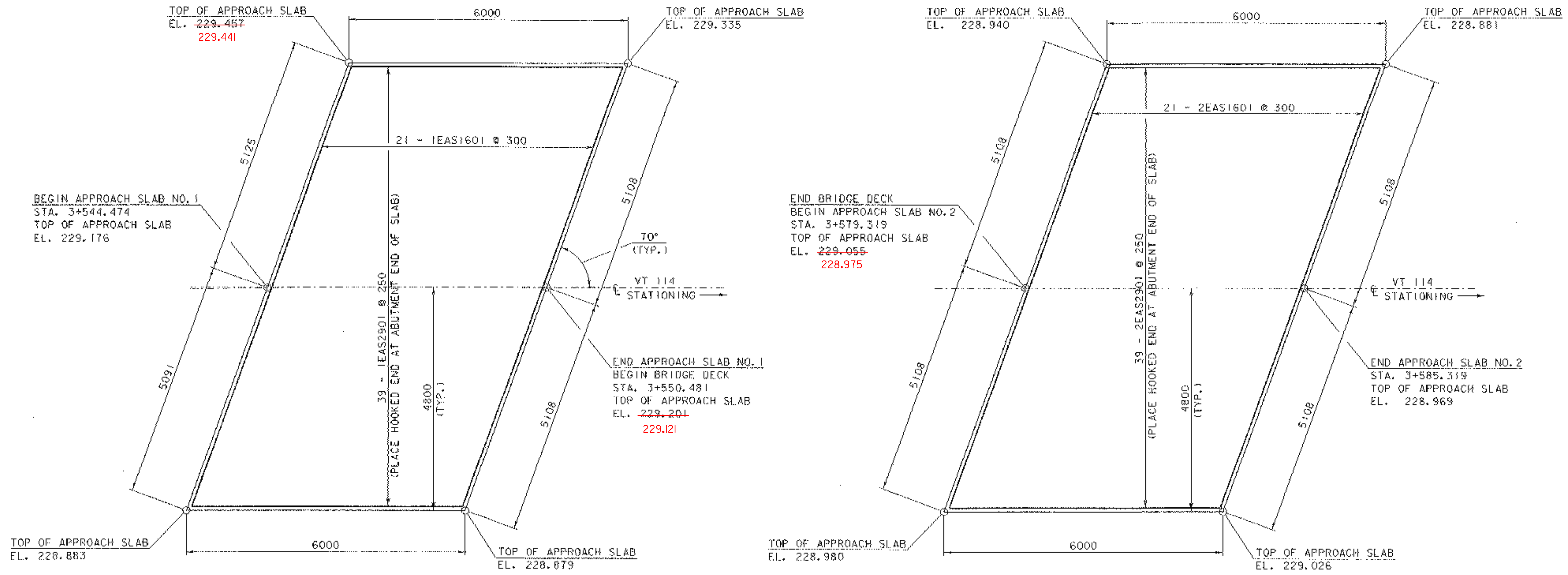
APPROACH SLAB PLAN
