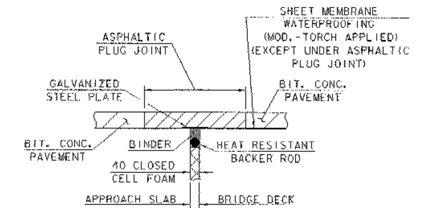
ASPHALTIC PLUG JOINT DETAIL AT EXPANSION END
