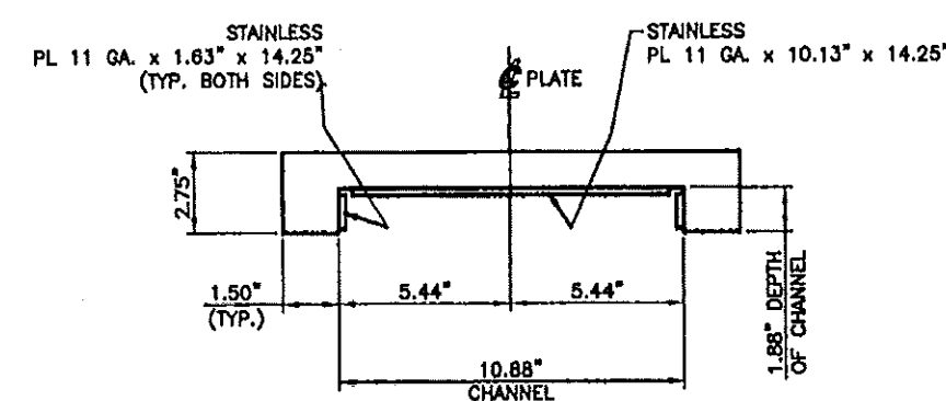
(4) CHANNELLED SLIDER PLATES w/SS FOR 267 KIP [1187 kN] GUIDED EXP. BRGS. PL 2.75" x 13.88" x 14.505"
