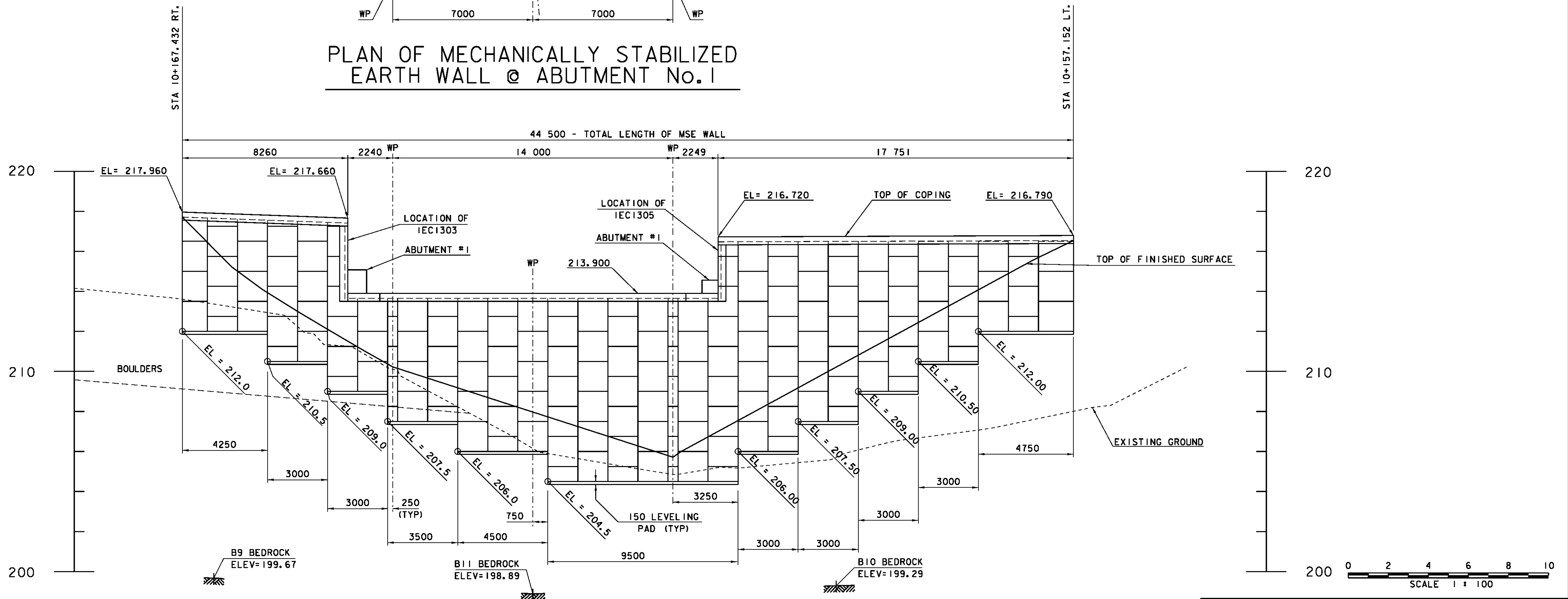
ELEVATION ALONG FACE OF MECHANICALLY STABILIZED EARTH WALL @ ABUTMENT NO. 1
