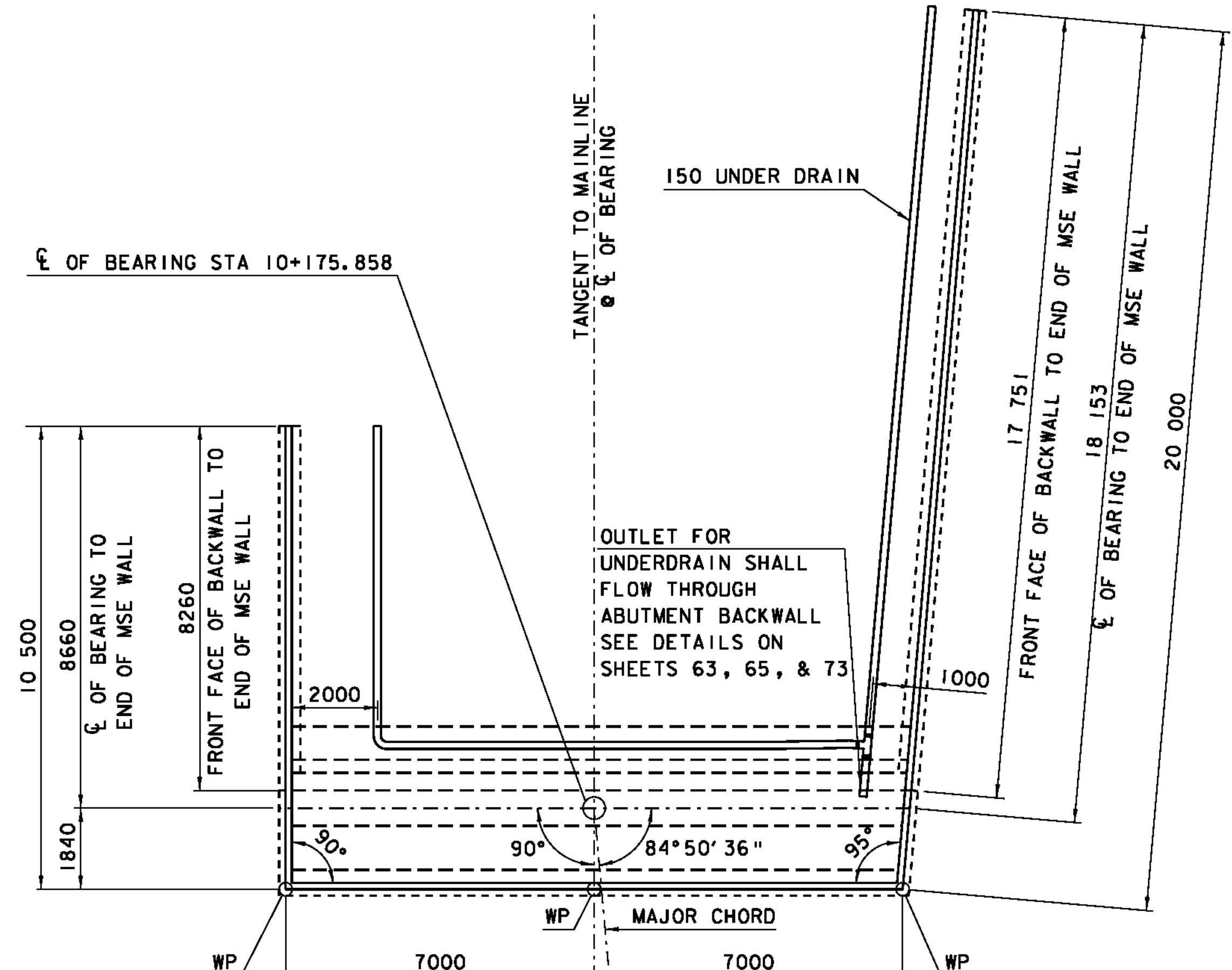
PLAN OF MECHANICALLY STABILIZED EARTH WALL @ ABUTMENT No. 1
