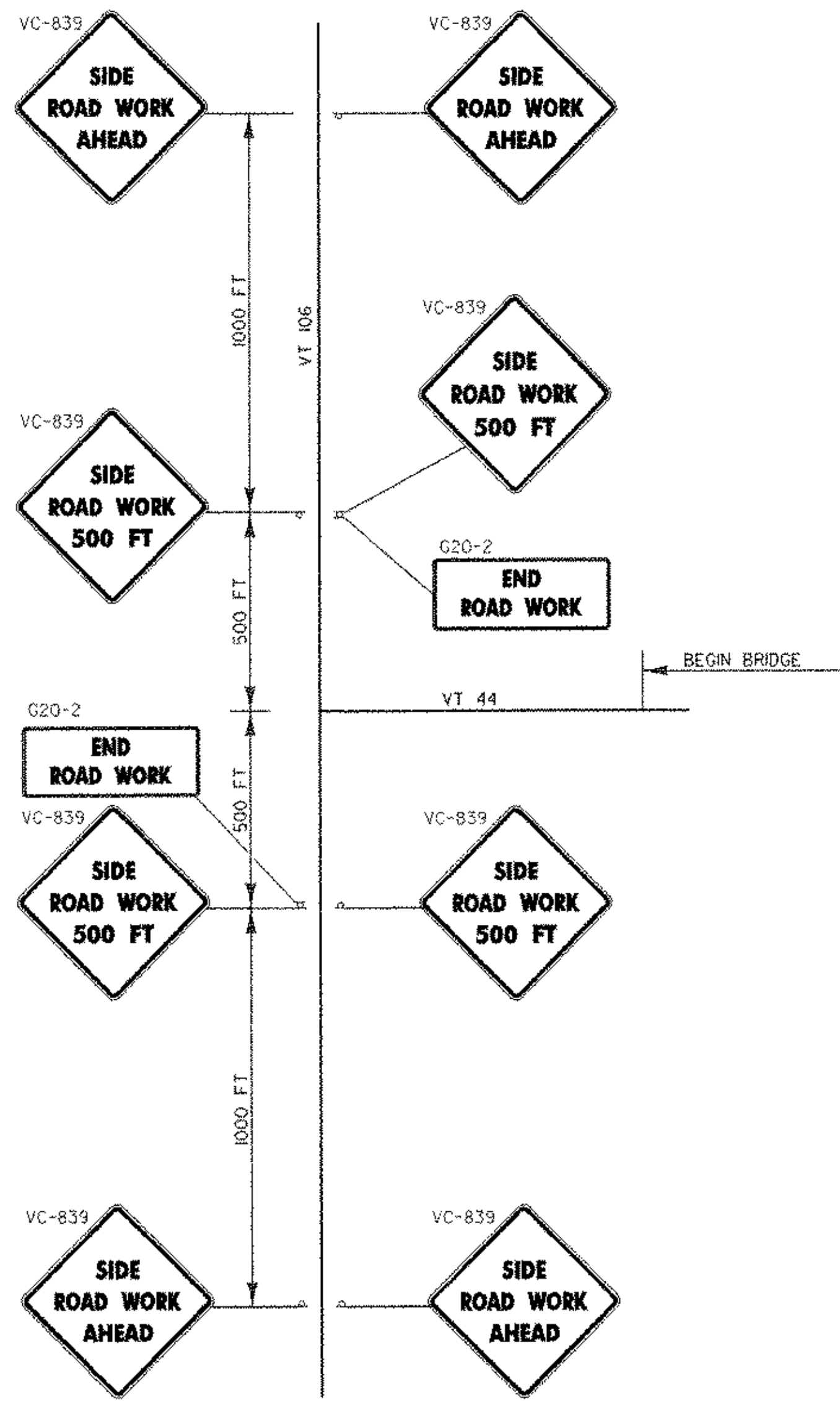
CONSTRUCTION APPROACH SIGNING (NOT TO SCALE)
