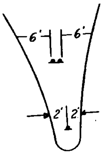
GORE SIGN PLACEMENT DETAIL
