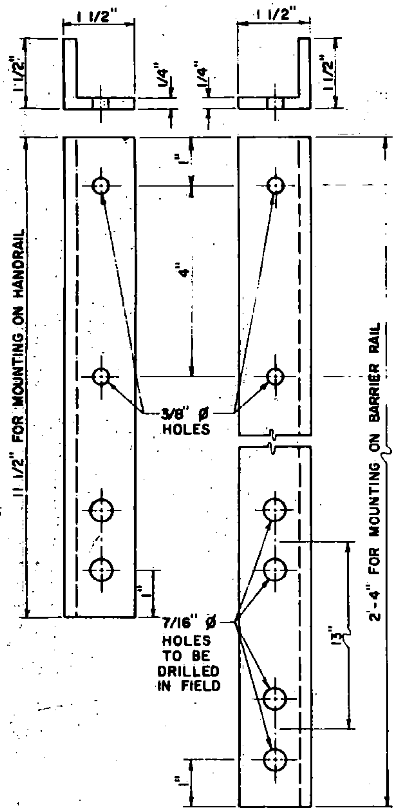
DETAIL "B" ALUMINUM ANGLE ASTMB - 308 ALLOY 6061 T6 SCALE 1" = 2"
