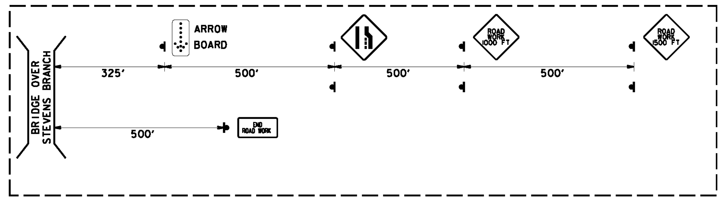
ADVANCED SIGNING ALONG ROUTE 62 (MIRROR FOR LEFT LANE CLOSURES)
