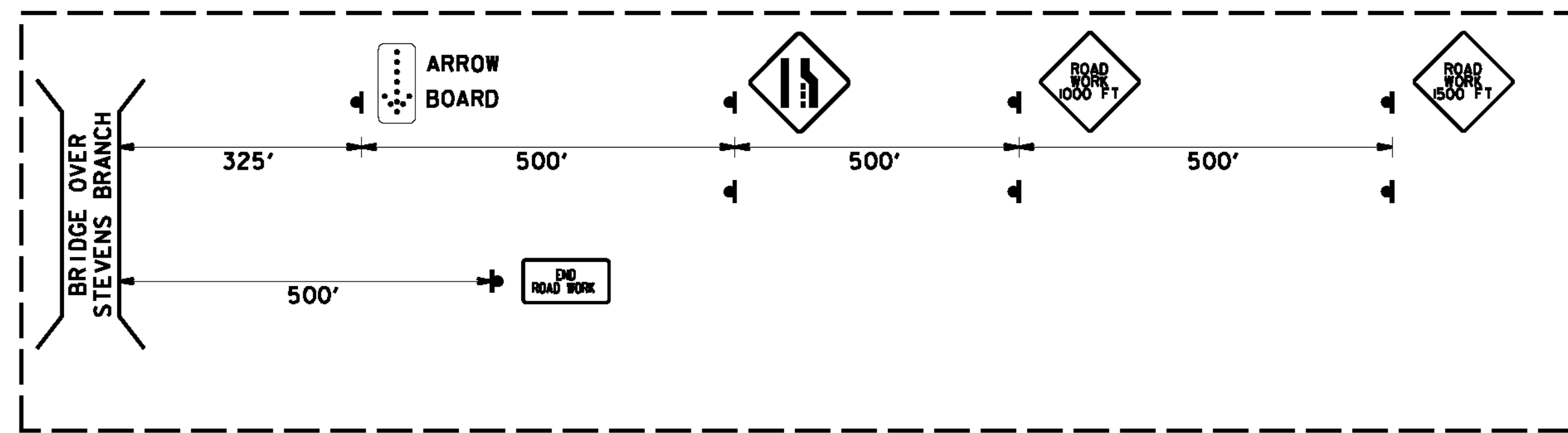
ADVANCED SIGNING ALONG ROUTE 62 (MIRROR FOR LEFT LANE CLOSURES)
