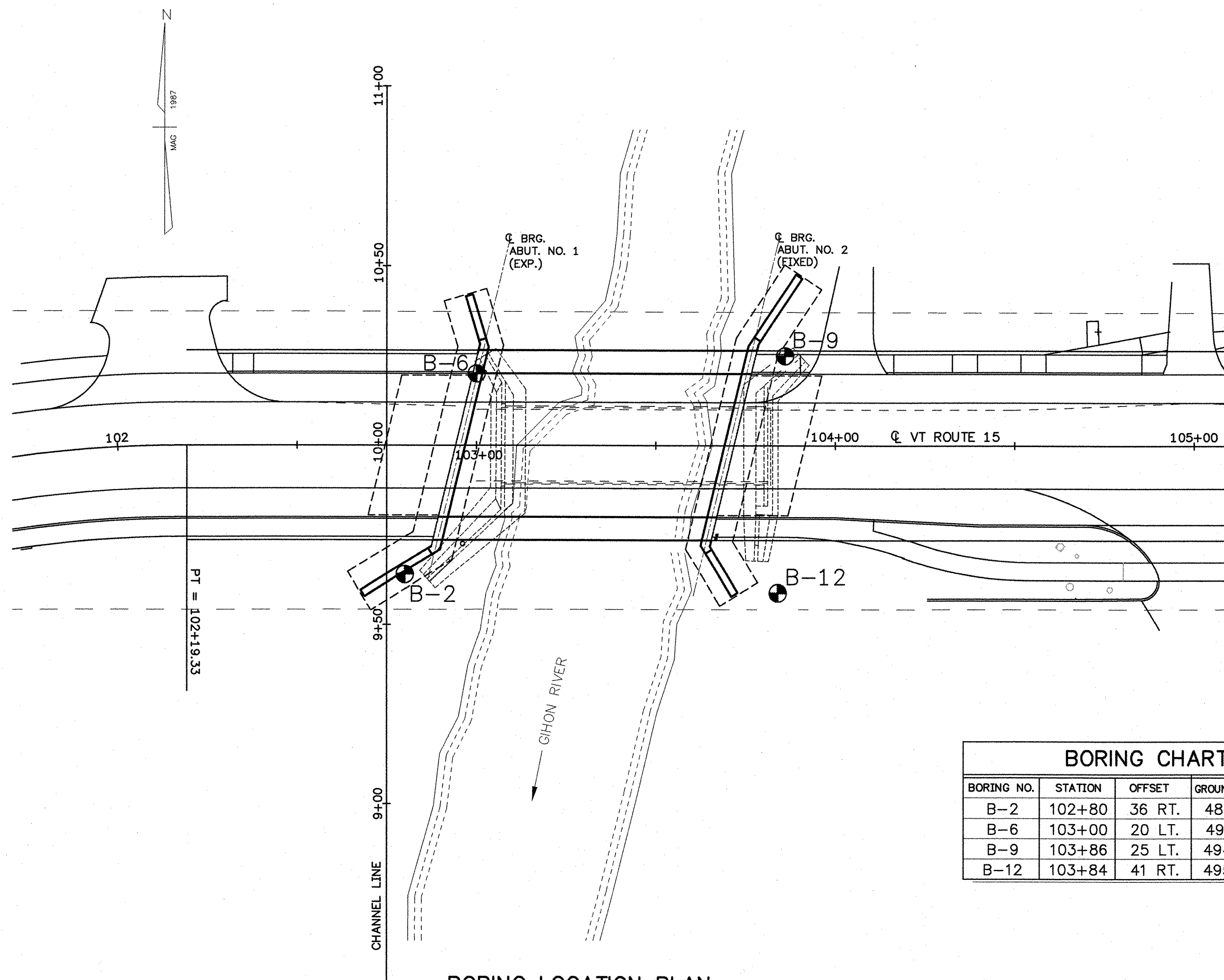
BORING LOCATION PLAN
