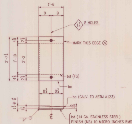
SOLE PLATES ~ MK. SP2 (PIER)
