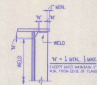
TYP. WELDING DETAIL
