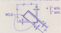
CROSSFRAME WELDING DETAIL
