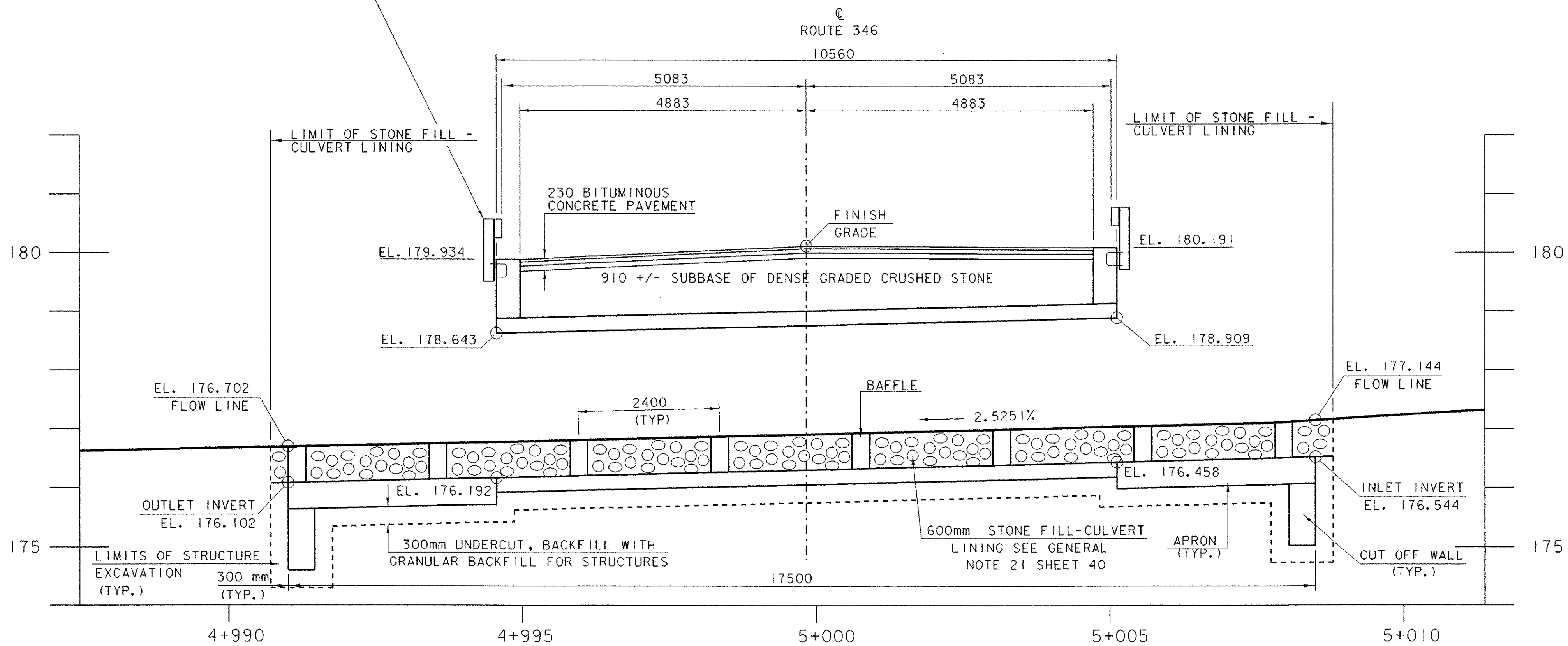
CHANNEL PROFILE ALONG \bar{C} BOX
