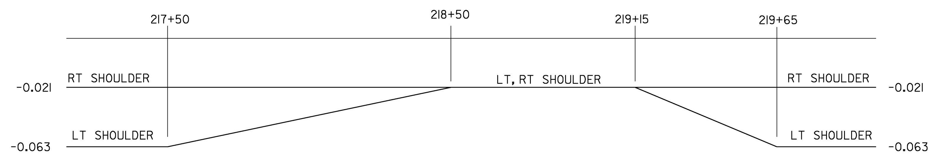
SHOULDER TRANSITION NTS
