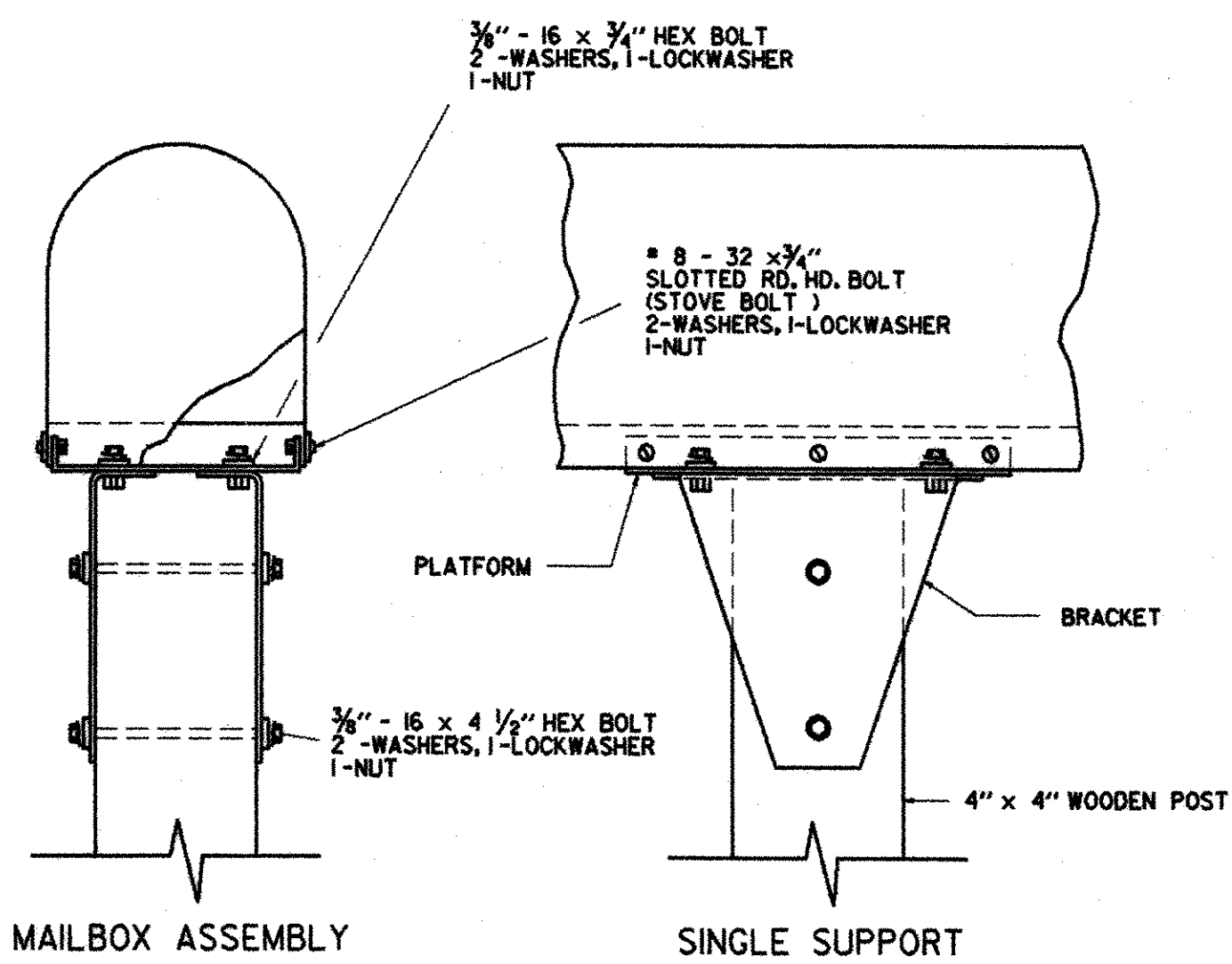
MAILBOX ASSEMBLY
