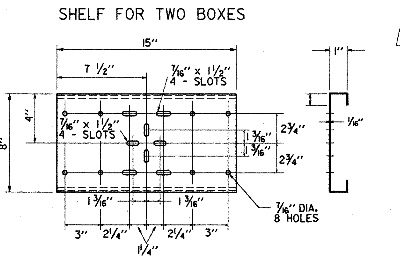
SHelf FOR TWO BOXES
