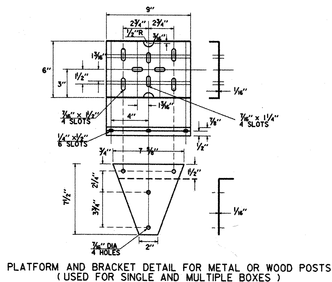
MAILBOX ASSEMBLY
