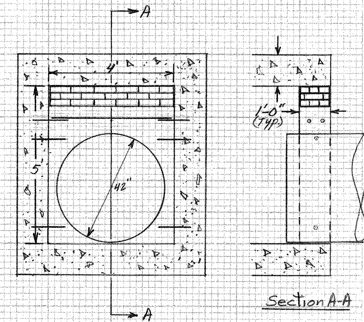
End Dam Detail (Typ) NTS
