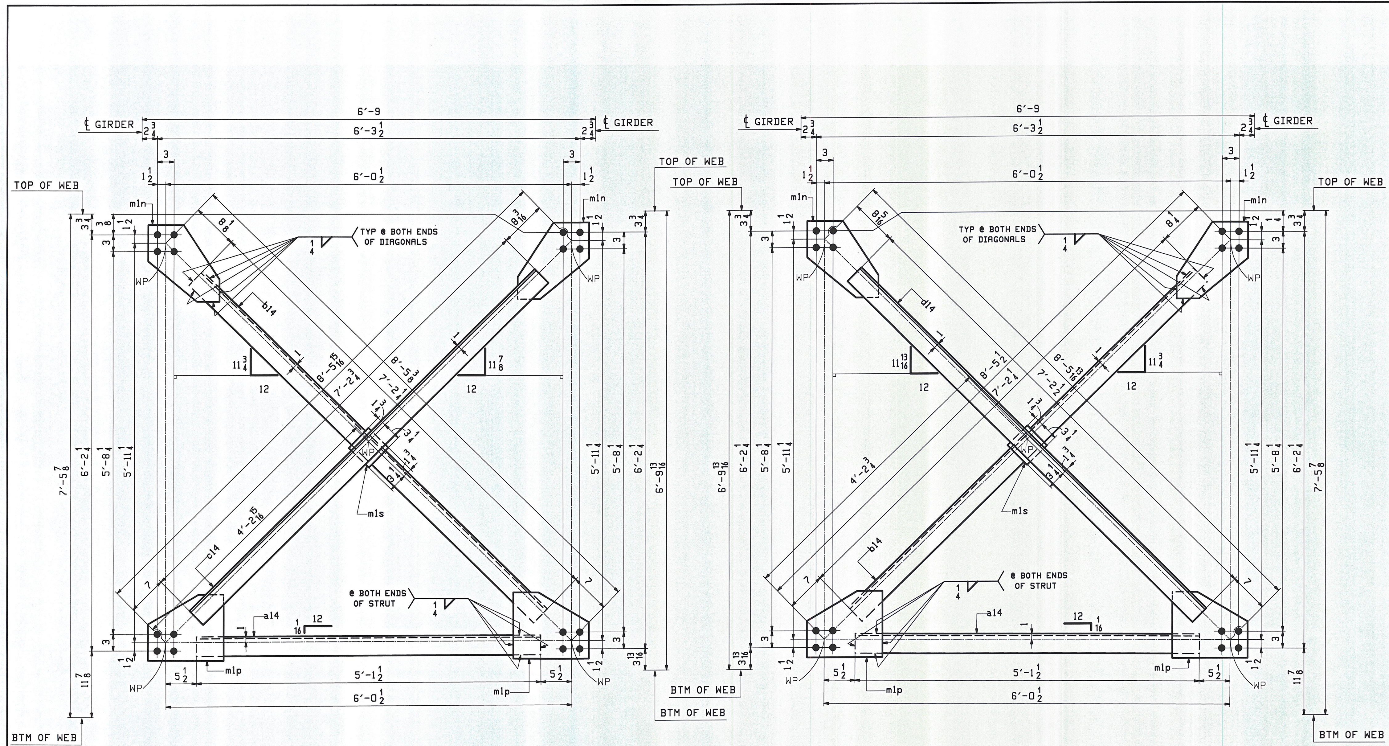
4 - INT CROSSFRAMES TYPE3 ~ 14CF1 LOOKING UPSTATION
