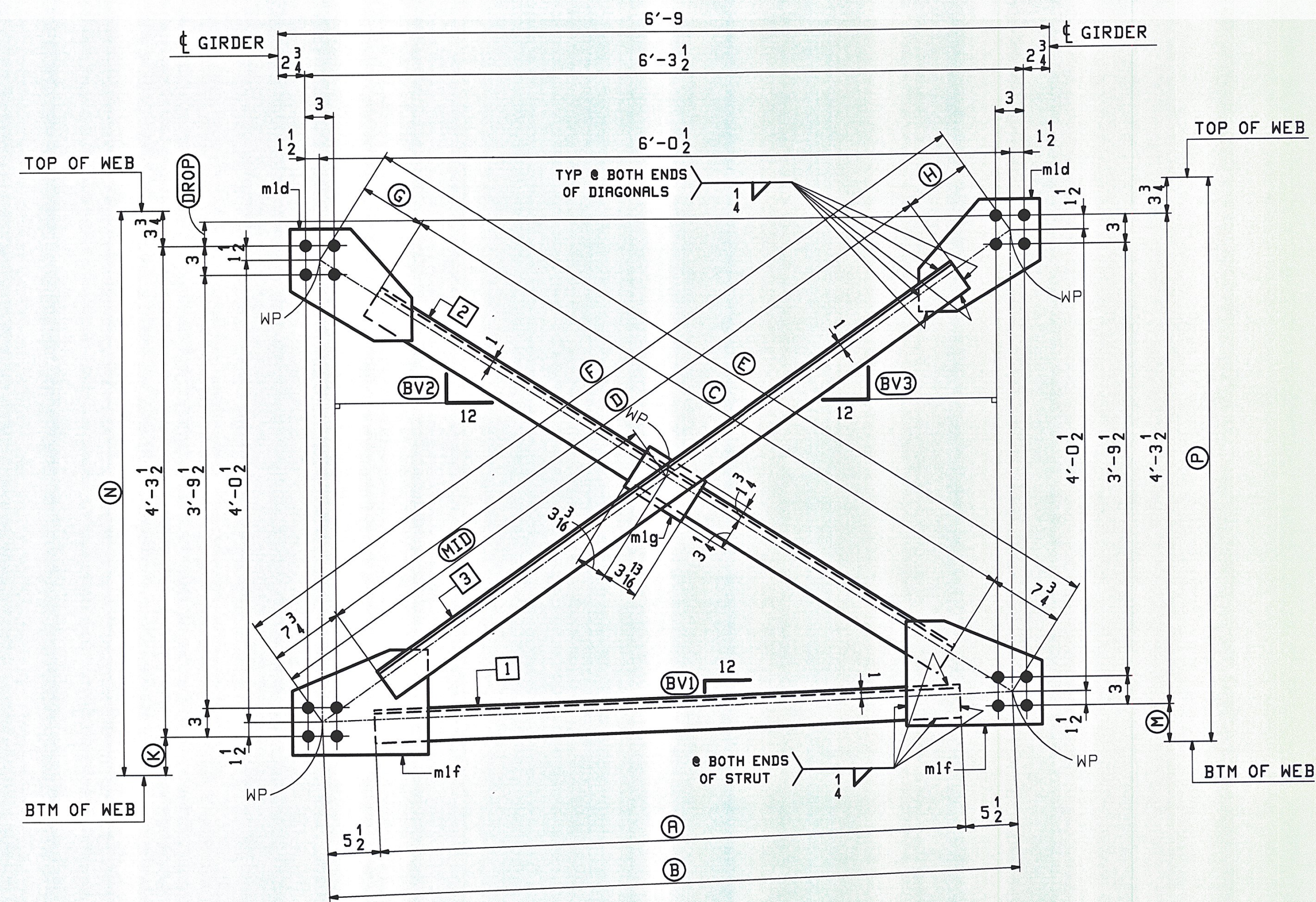
INT CROSSFRAMES - TYPE "CF1" LOOKING UPSTATION
