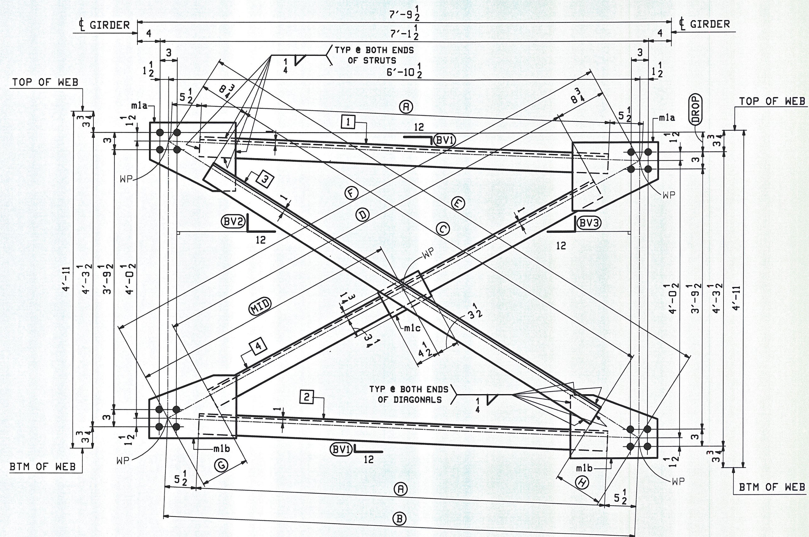
END CROSSFRAMES LOOKING TOWARDS BACKWALL
