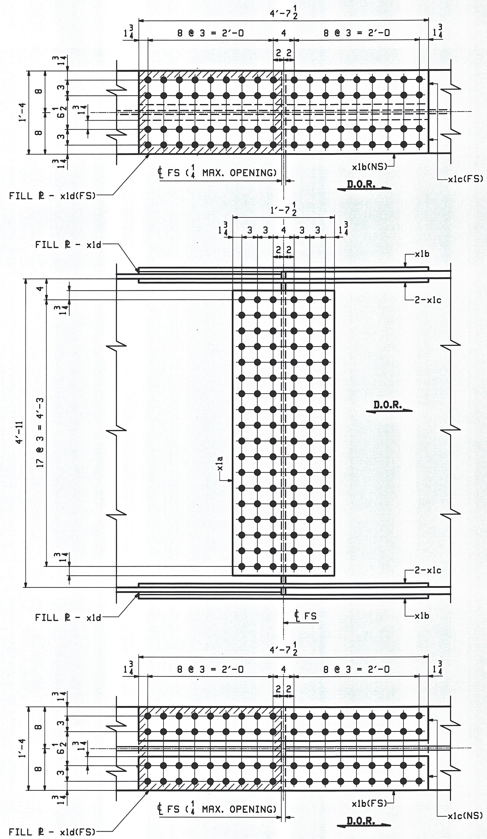
10 - FIELD SPLICE DETAIL - X1M1 FIELD SPLICE 1 & 2 (FOR F.S. 2 ROTATE 180°)
