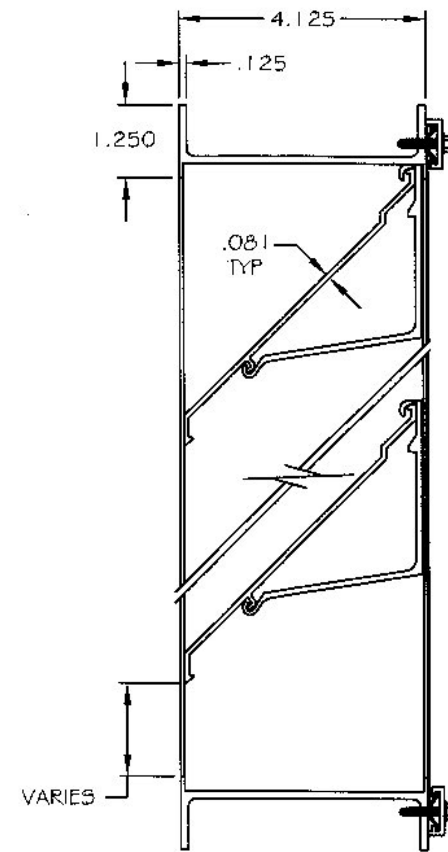
HEAD & SILL DETAIL
