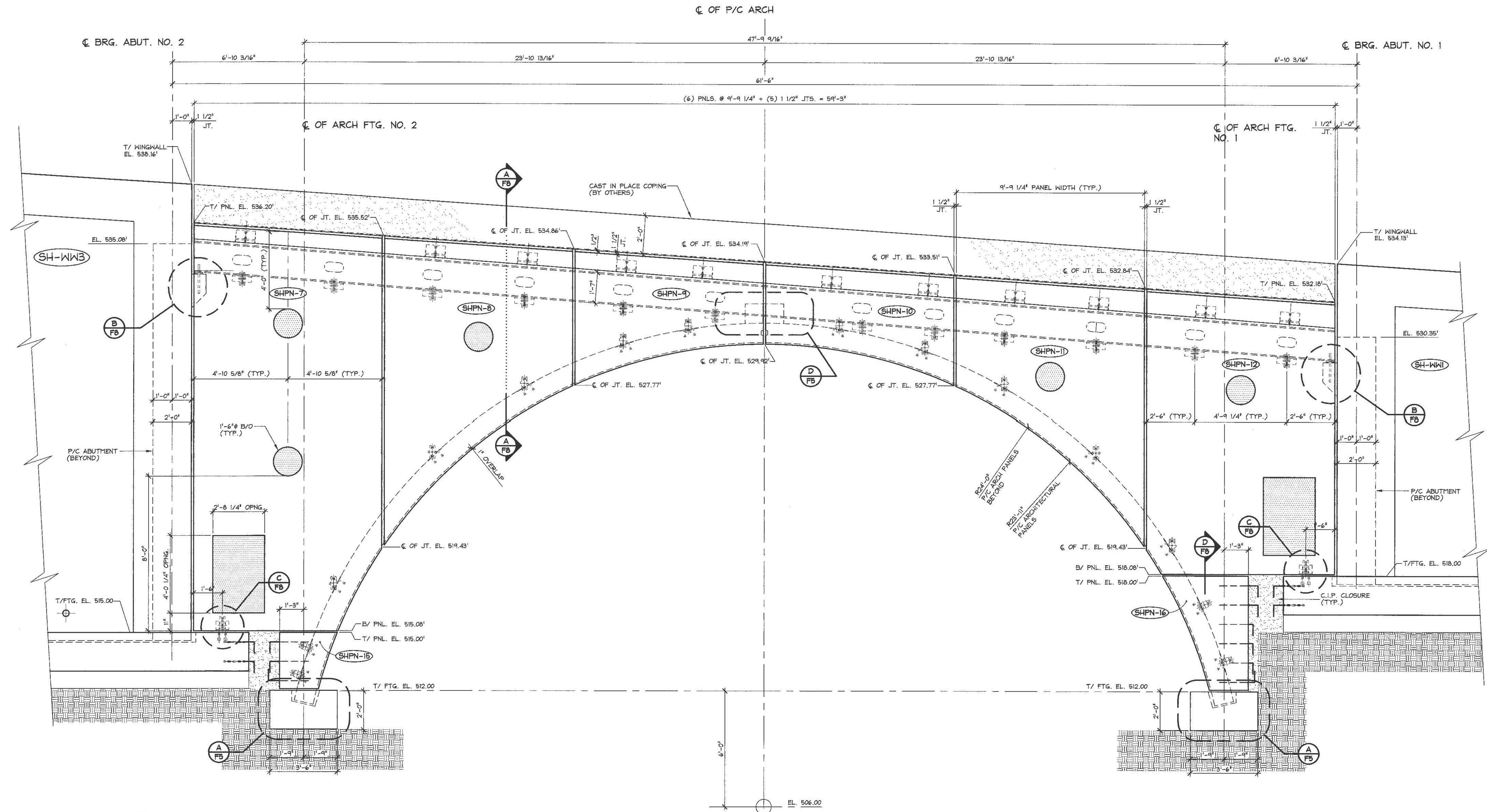
2 EAST ELEVATION OF PRECAST ARCHITECTURAL PANELS F7 3/8" = 1'-0"
