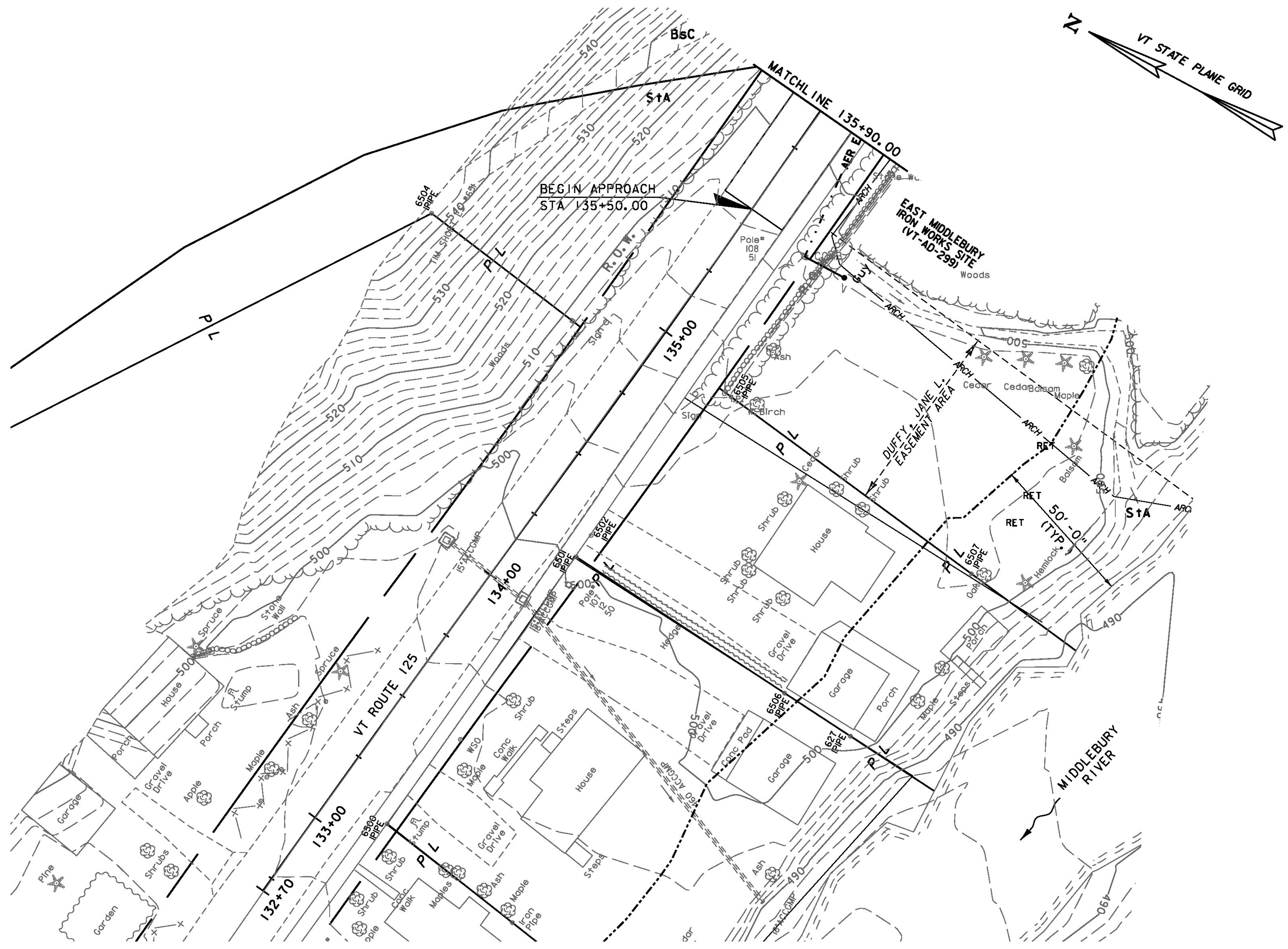
PLAN SCALE 1" = 20'-0" 20 0 20
