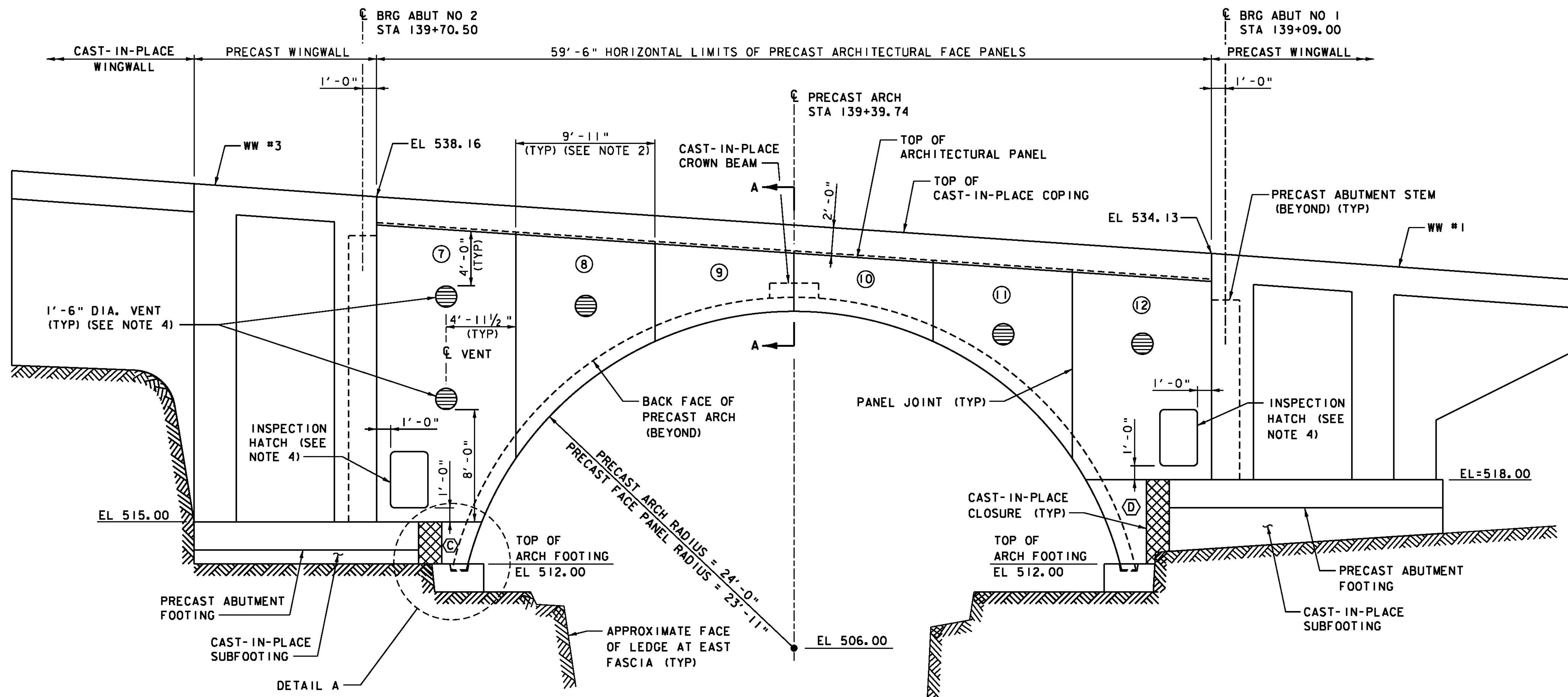
EAST PRECAST ARCHITECTURAL PANEL ELEVATION SCALE 1/4" = 1'-0"
