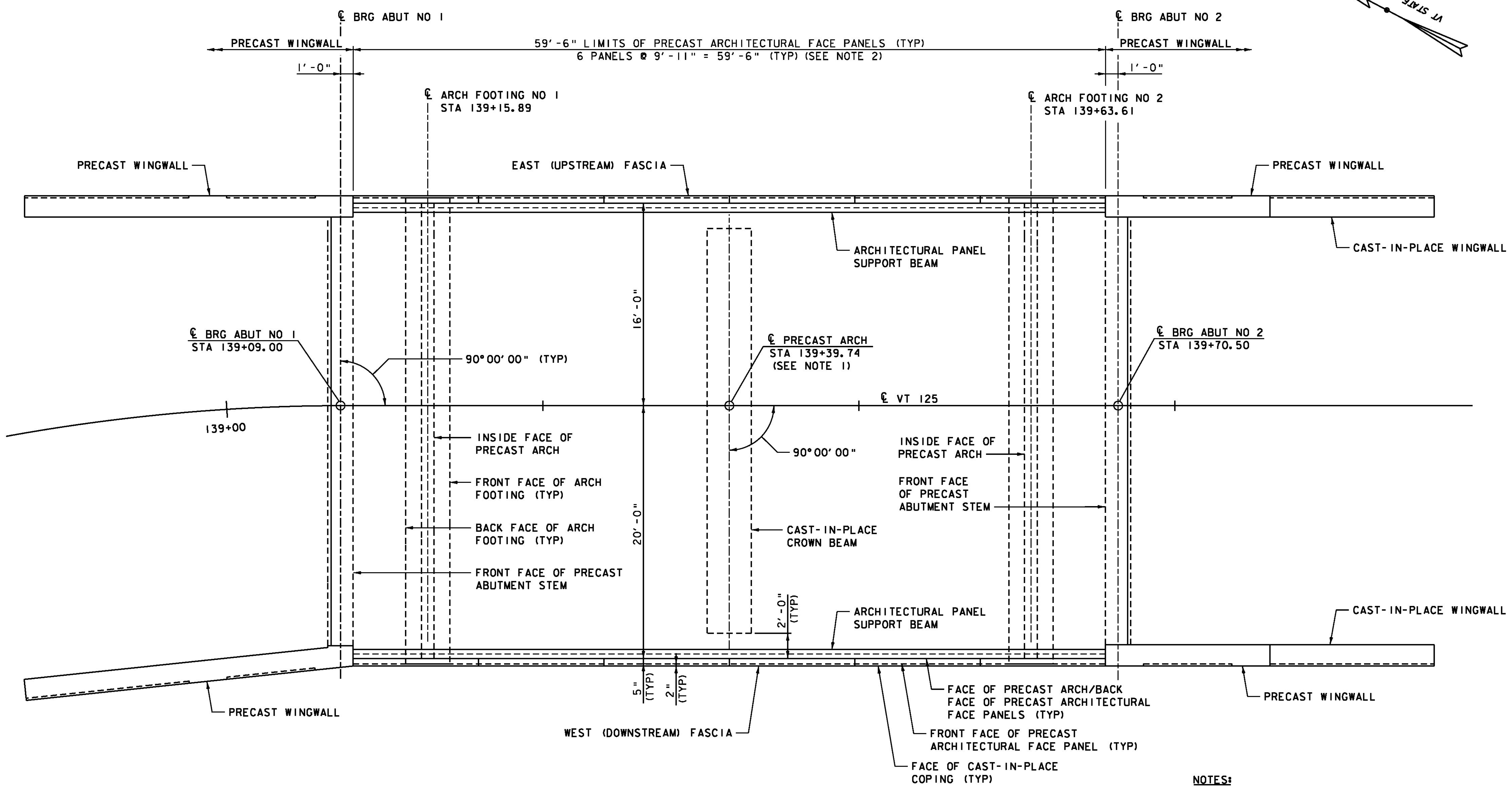
PRECAST ARCHITECTURAL PANEL PLAN SCALE 1/4" = 1'-0"
