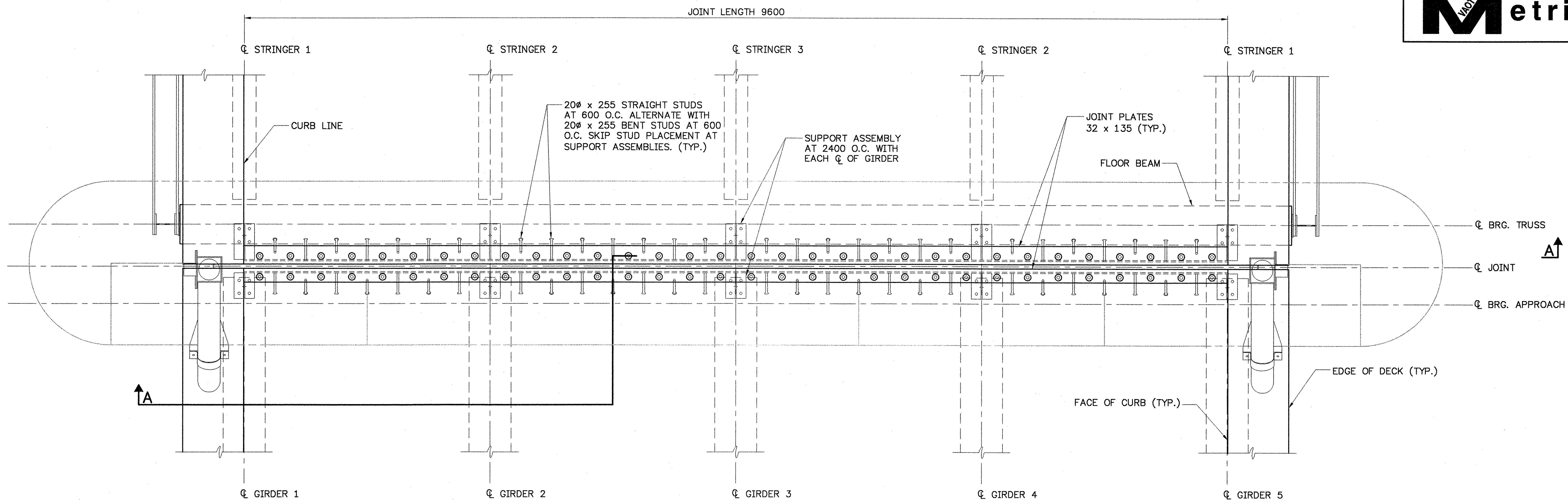
PLAN OF EXPANSION JOINT SCALE 1:20
