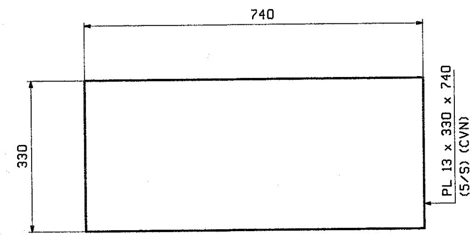
60 ~ GUSSET PL ~ mlf CENTER
