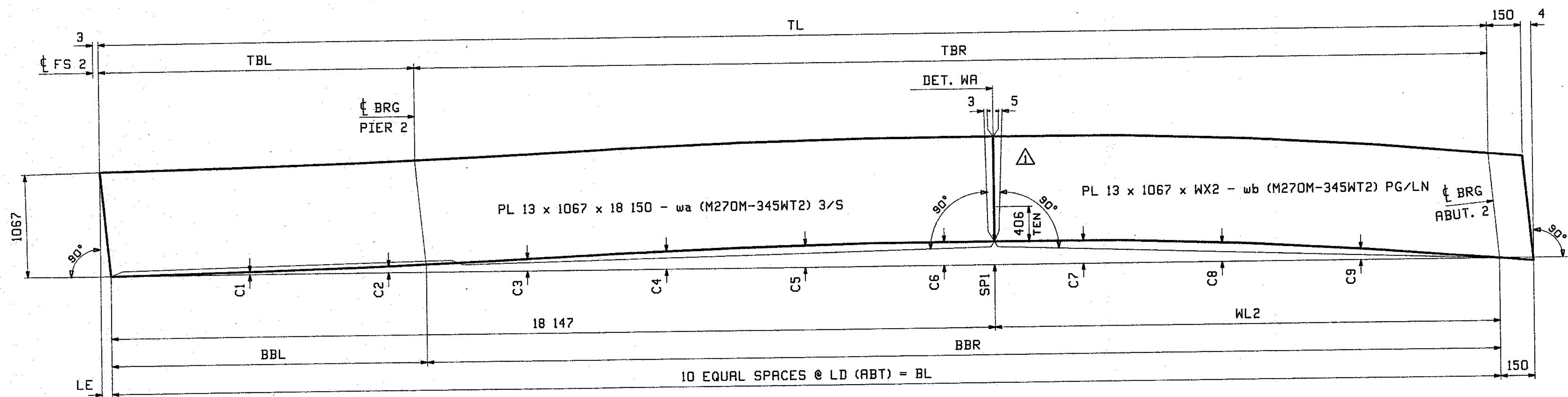
CAMBER DIAGRAM FOR 9G1C, 10G2C, 11G3C & 12G4C
