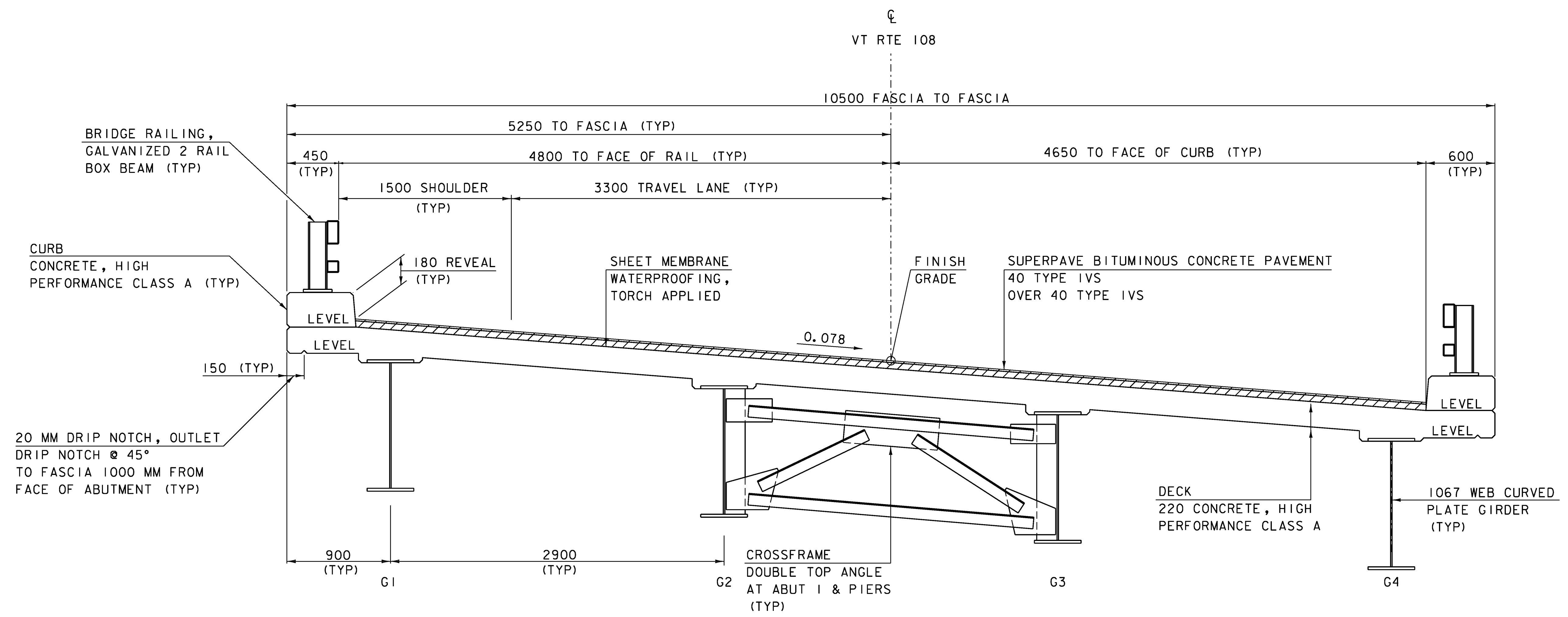
TYPICAL BRIDGE SECTION
