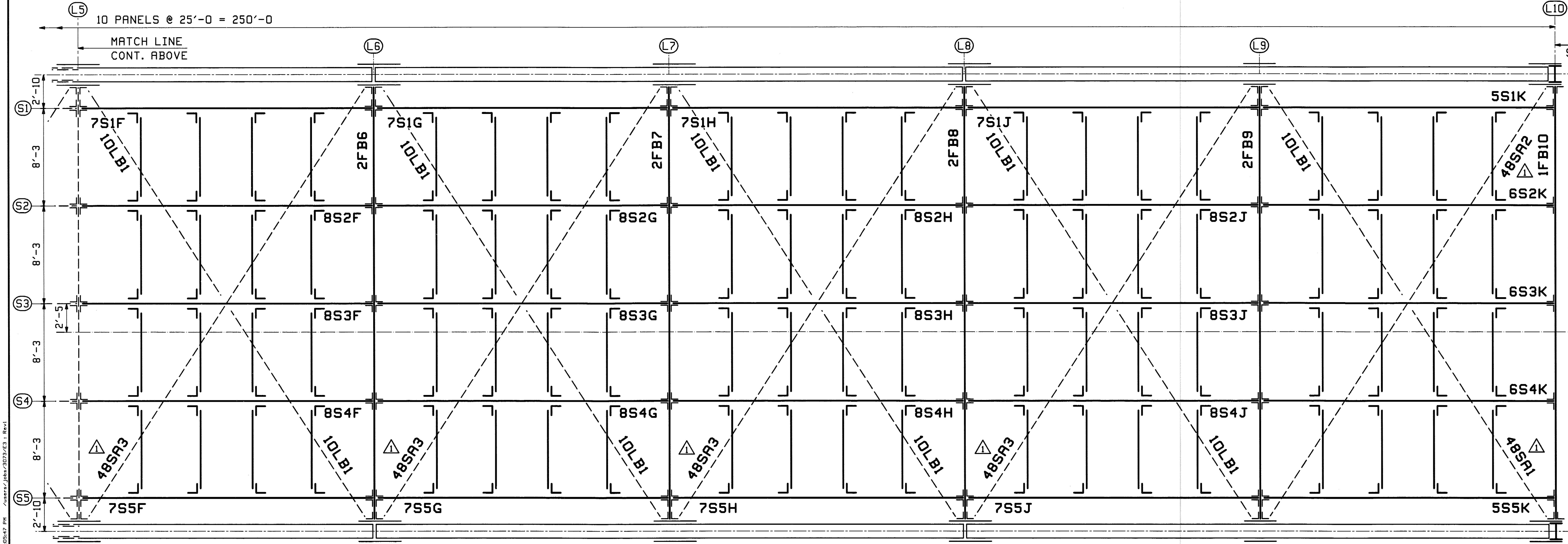
LOWER CHORD FRAMING PLAN
