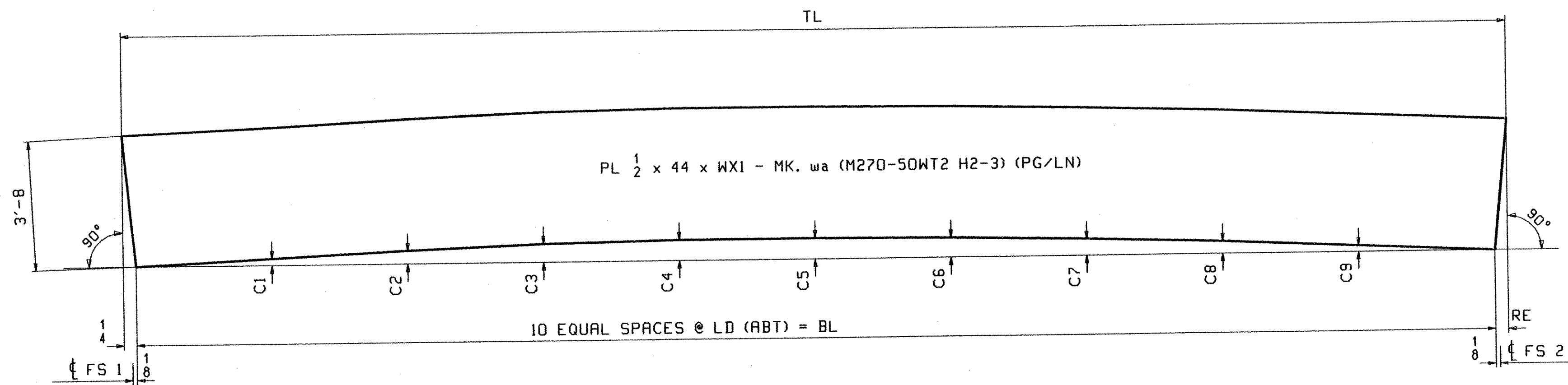
WEB CUTTING DIAGRAM FOR G1B THRU G6B
