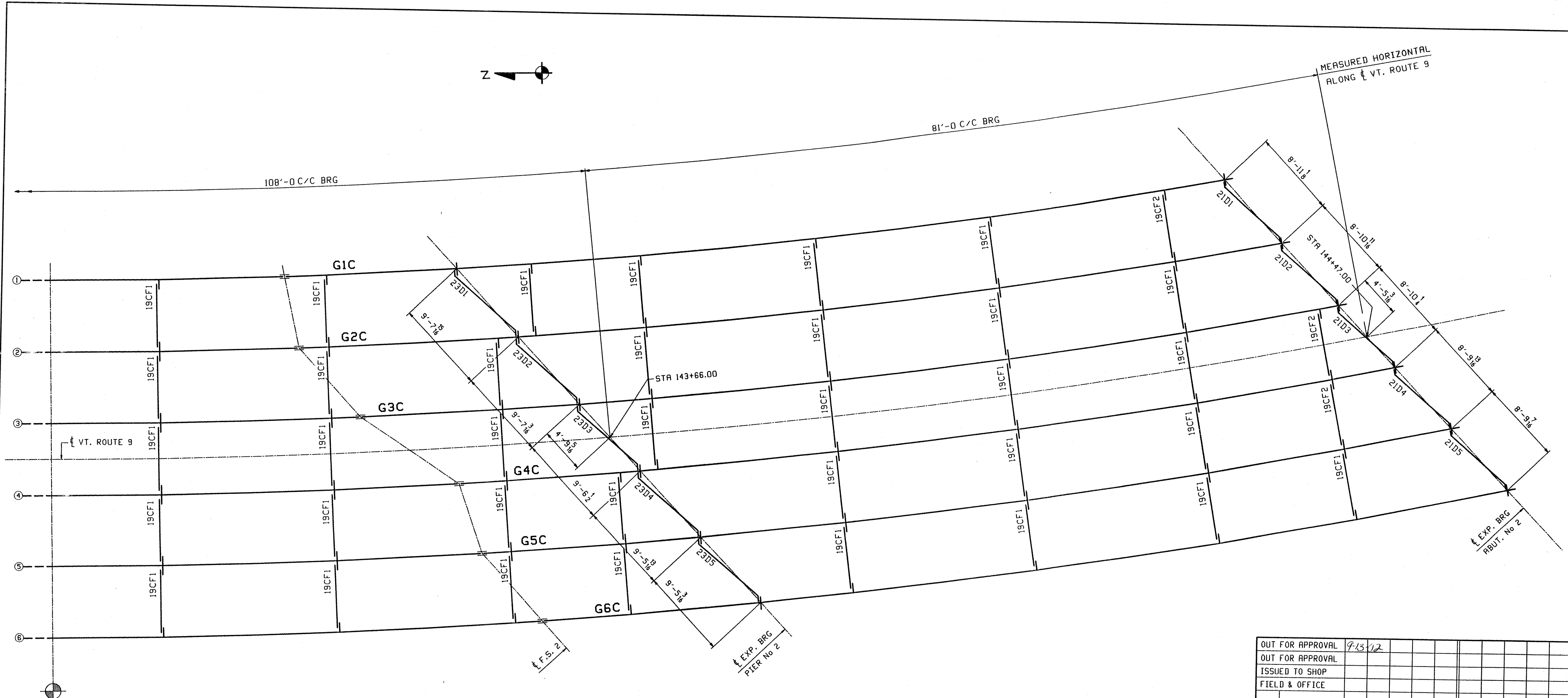
FRAMING PLAN FOR BRIDGE 25B
