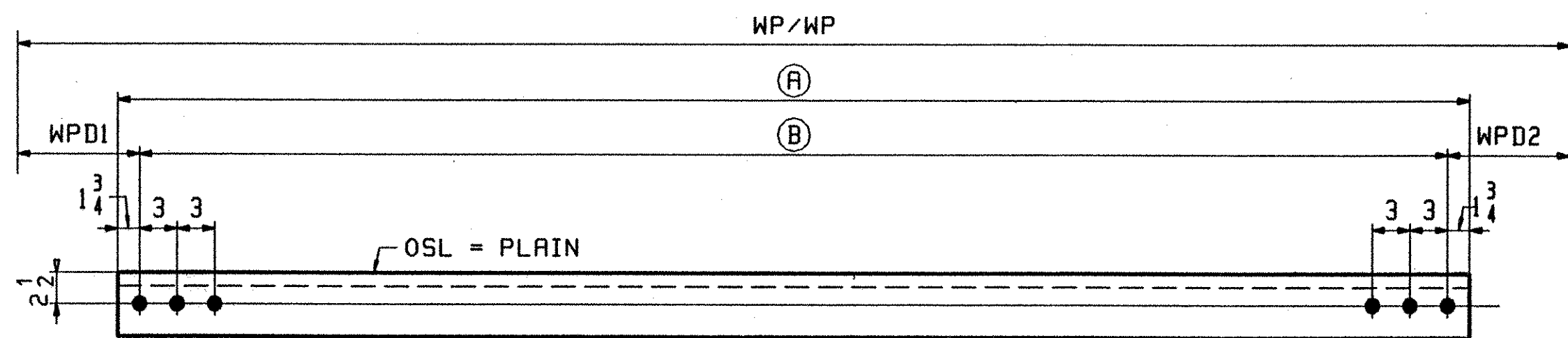
LATERAL BRACING
