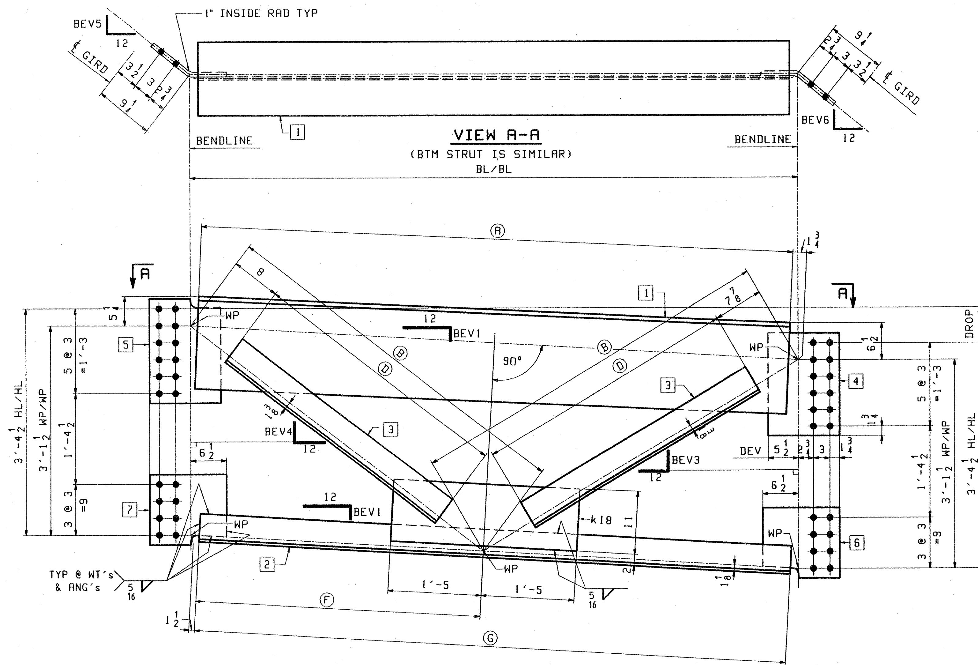
ABUTMENT CROSSFRAME TYPE C1 (ALL PRINTED)
