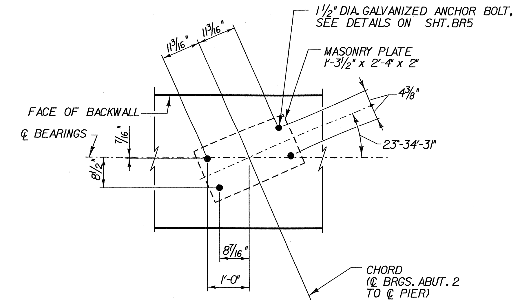
PLAN-ANCHOR BOLT LAYOUT-ABUTMENT 2
