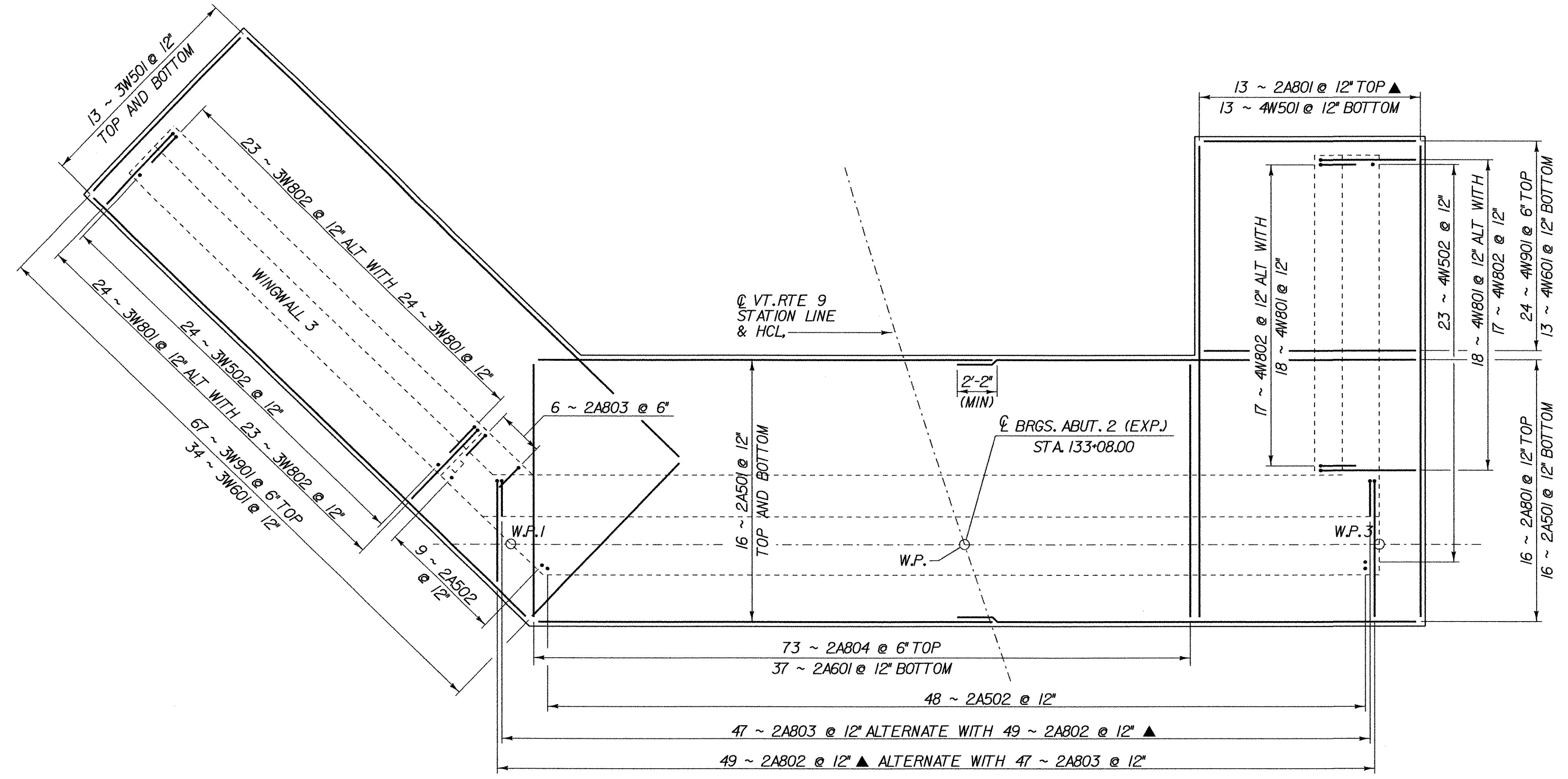
ABUTMENT 2 FOOTING REINFORCING PLAN - BR 25A
