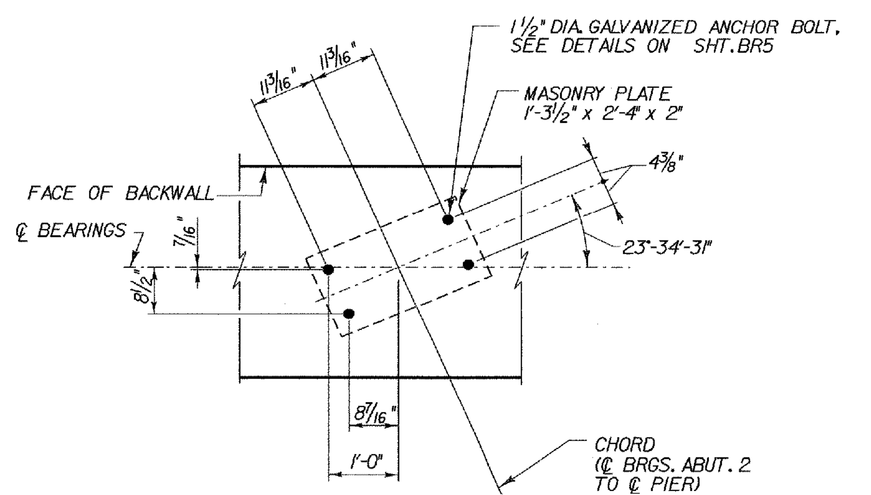
PLAN-ANCHOR BOLT LAYOUT-ABUTMENT 2 SCALE 3/4" = 1'-0"
