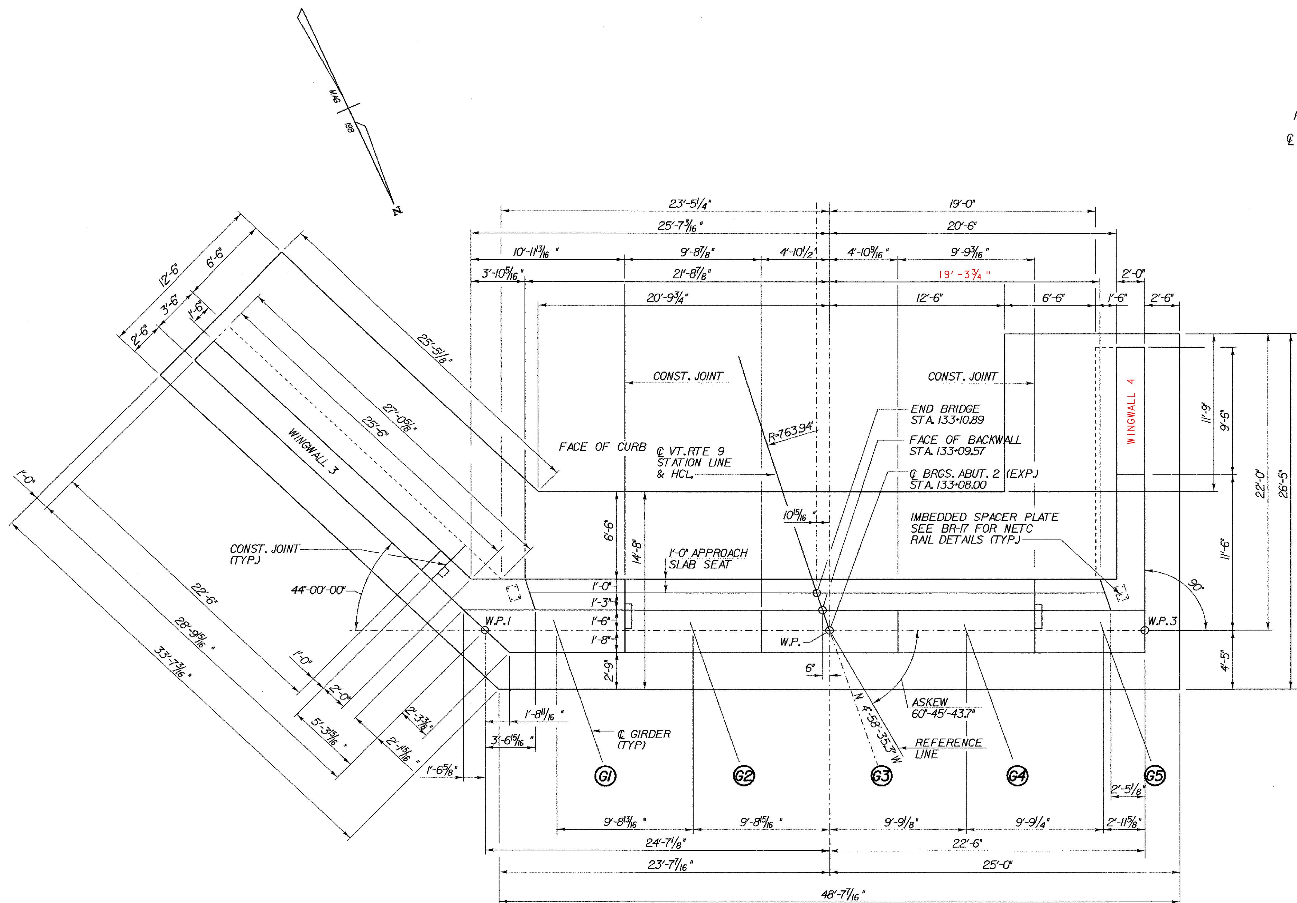
ABUTMENT 2 REDESIGN PLAN - BR 25A SCALE 1/4" = 1'-0"
