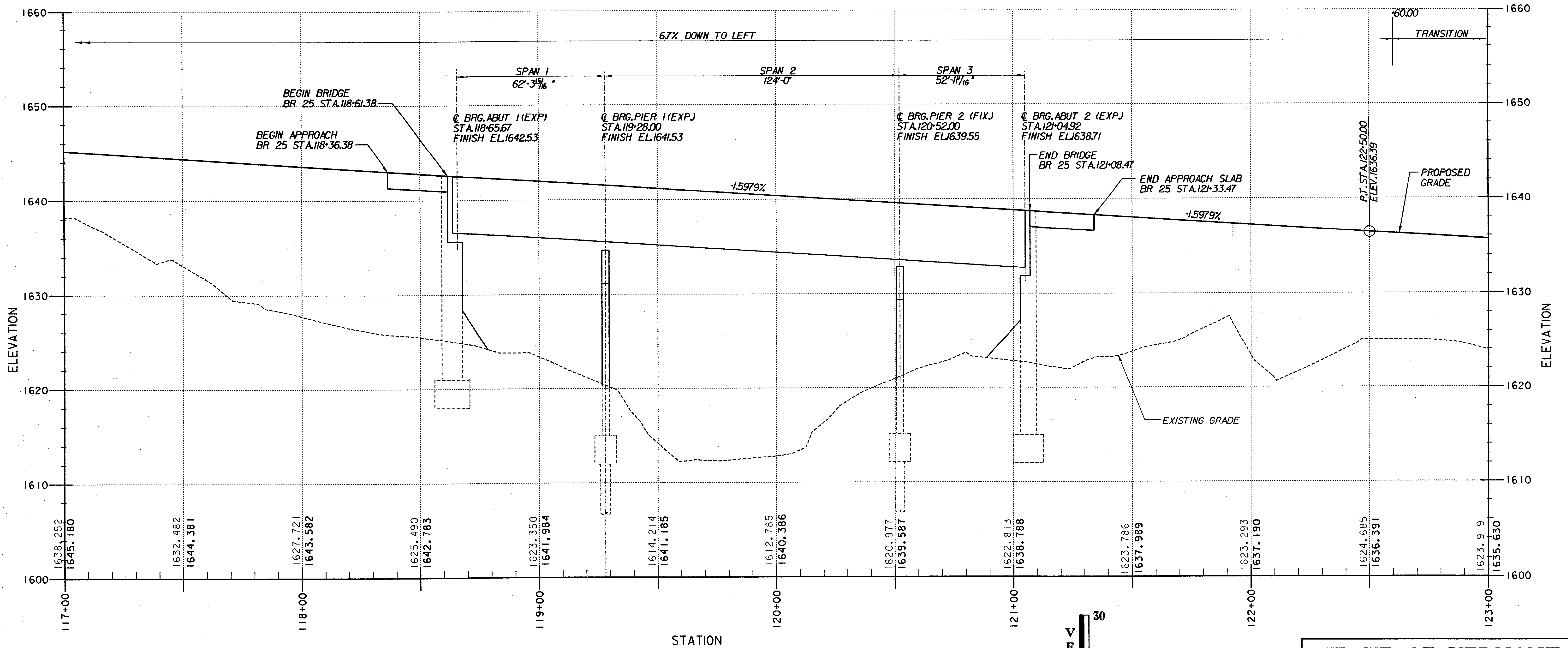
PROFILE - VT. RTE. 9 OVER DEERFIELD RIVER - BR 25
