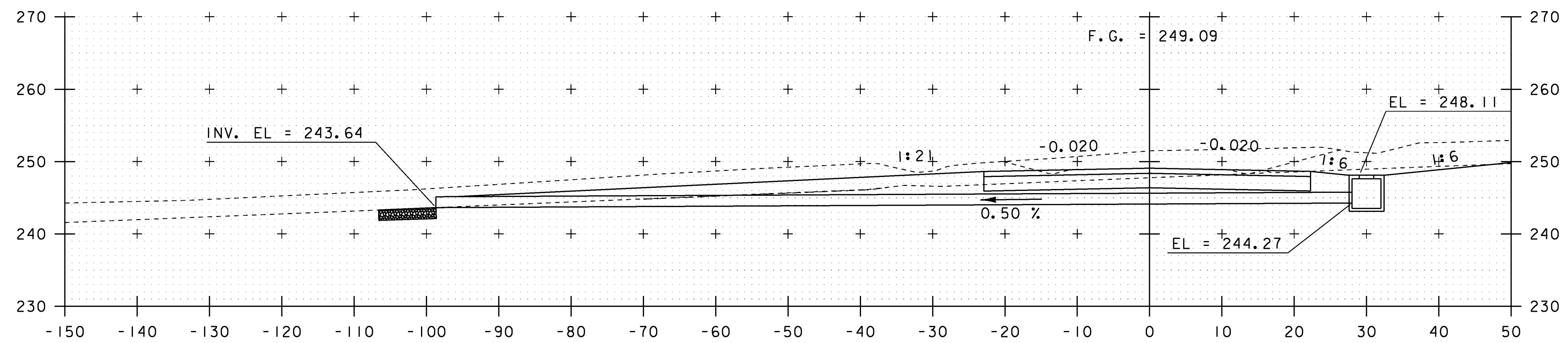
STATE PARK ROAD SECTION A-A
