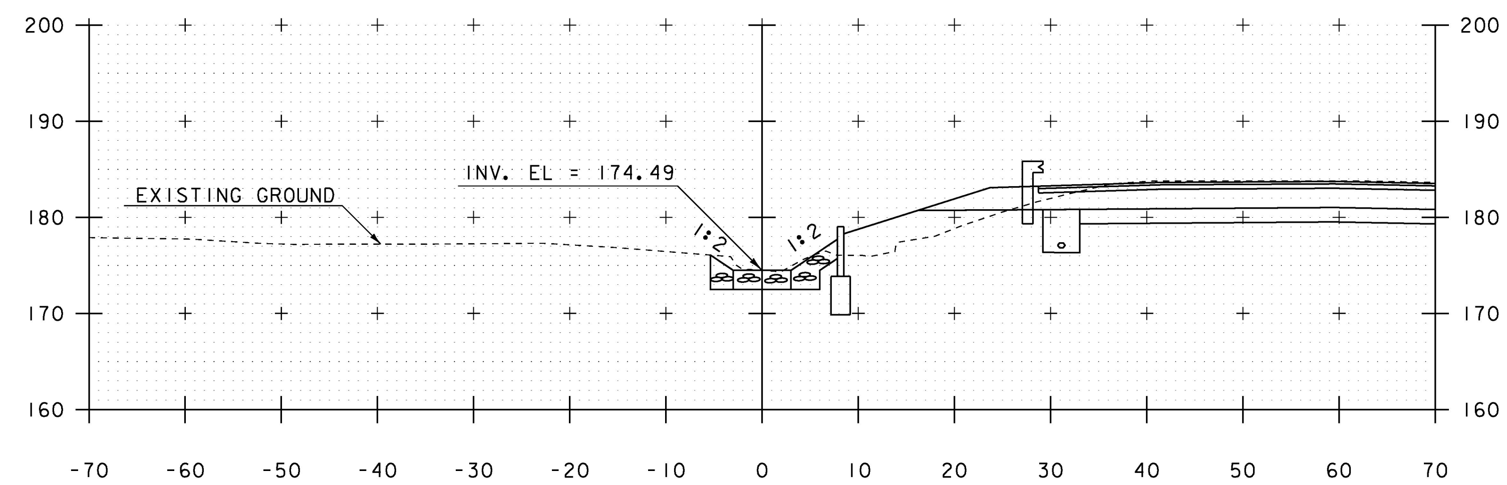
60+39.78 END CHANNEL WORK
