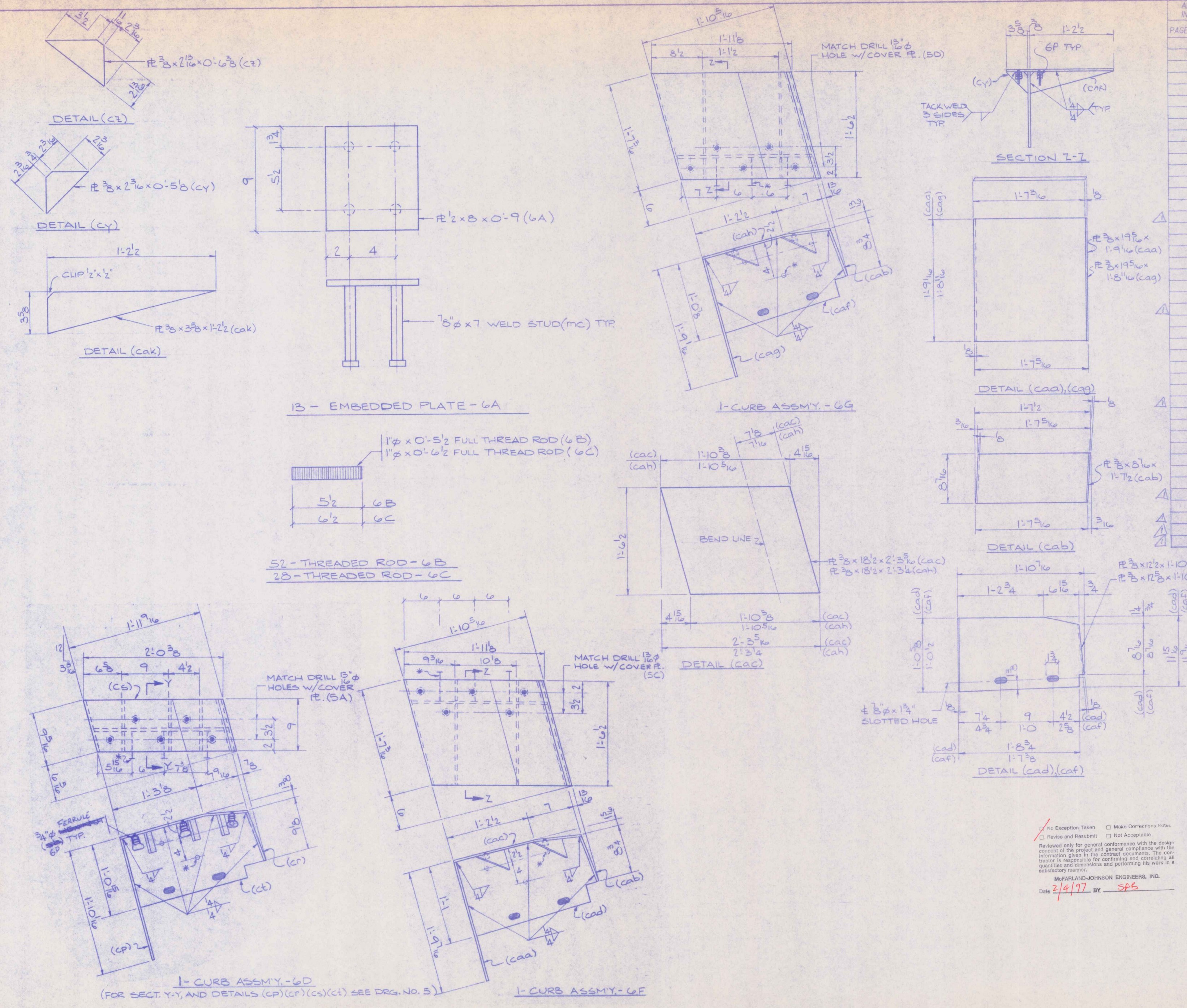
DETAIL (6O), (6P)
