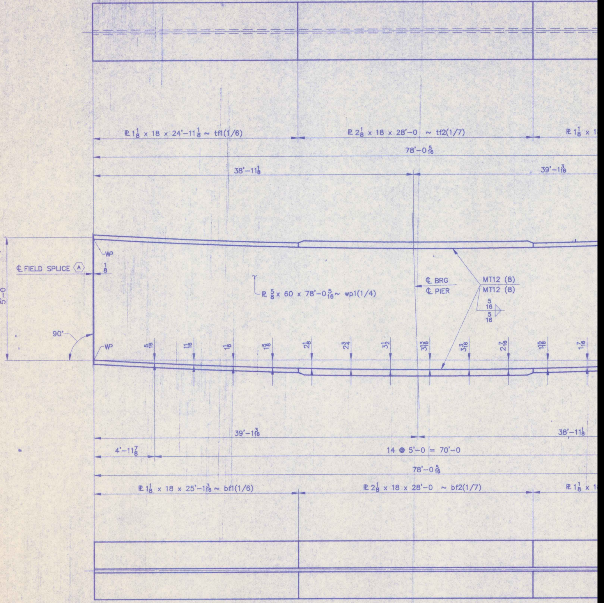
CAMBER DIAGRAMS ~ G1B THRU G7B
